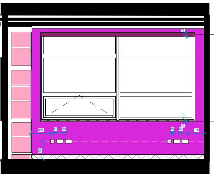
E CC-00-032 - Meeting Room - Elevation - E 1 : 50
