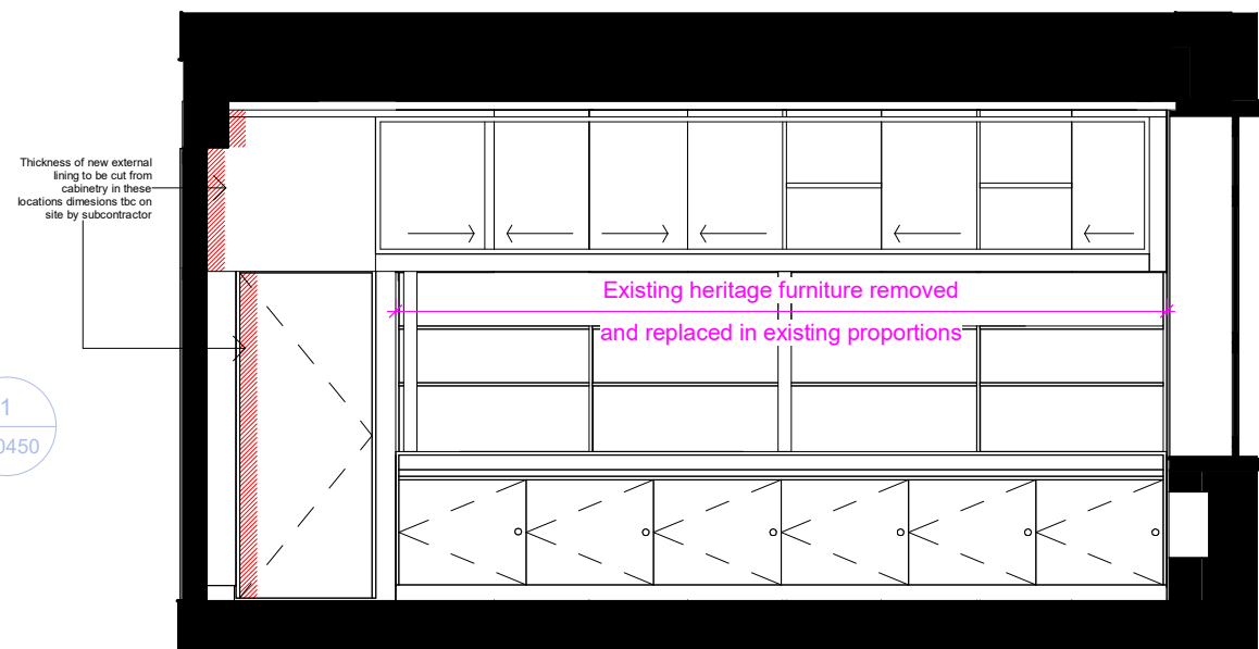
N-E CC-00-032 - Meeting Room - Cabinet existing 1 : 50
