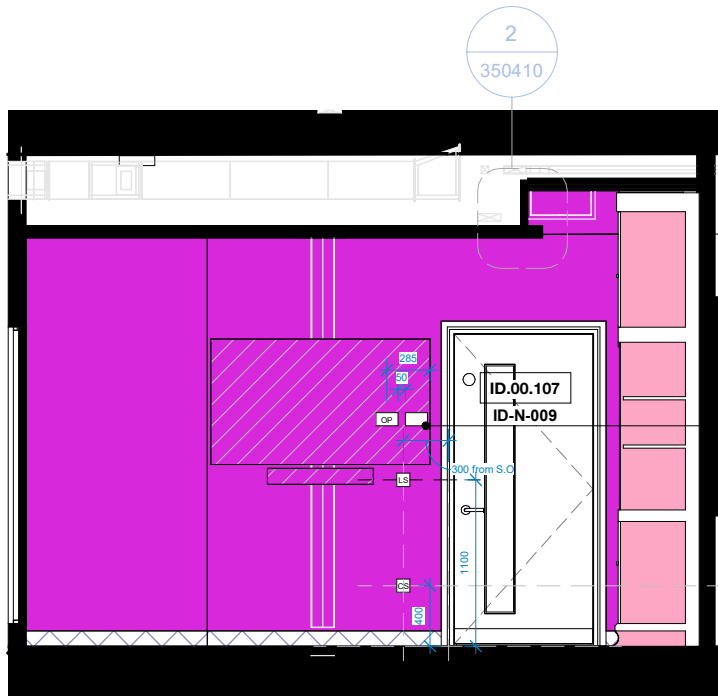
W CC-00-032 - Meeting Room - Elevation - W 1 : 50
