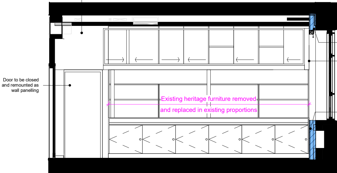
N-P CC-00-032 - Meeting Room - Cabinet Proposed positions 1 : 50
