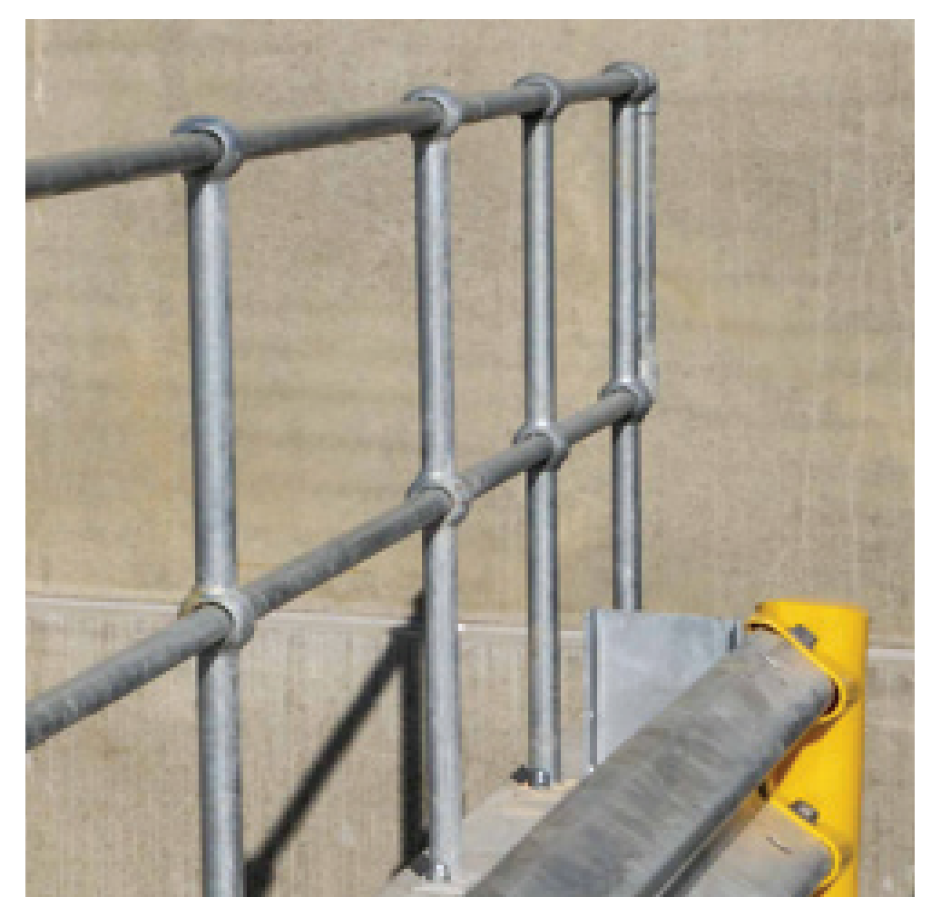
8 EXTERNAL RAMPs AND STEPS GUARDING, HANDRAILS GAL VANISED STEEL 1100mm HEIGHT ABOVE GROUND
