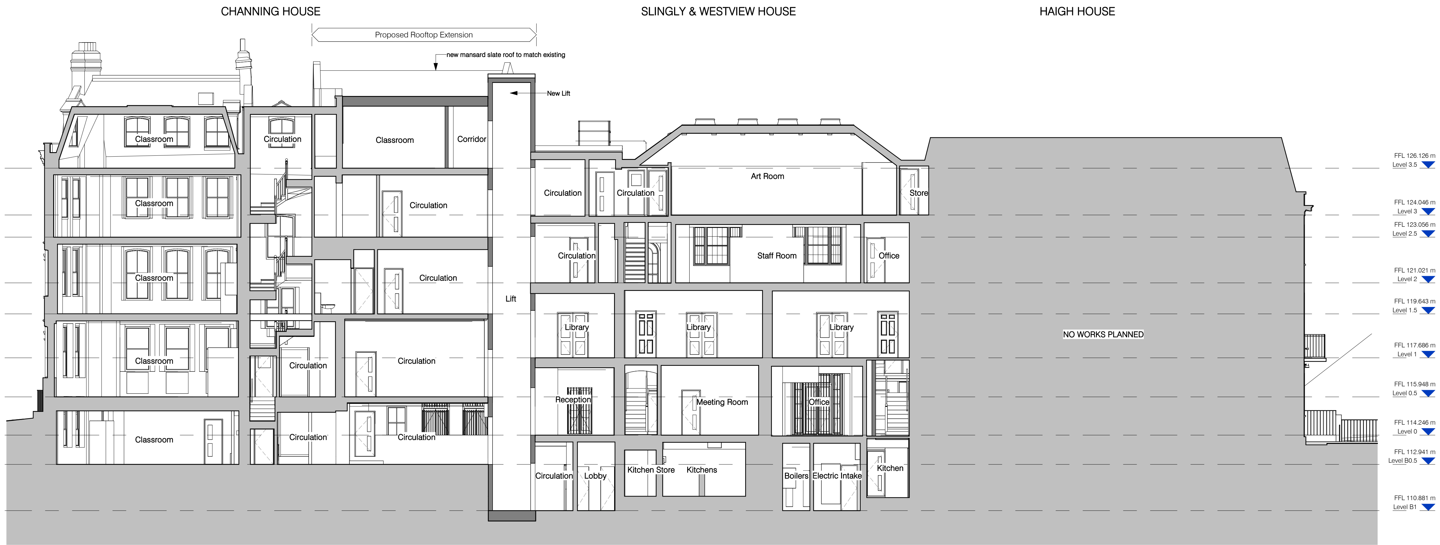
Proposed Section A 1:100
