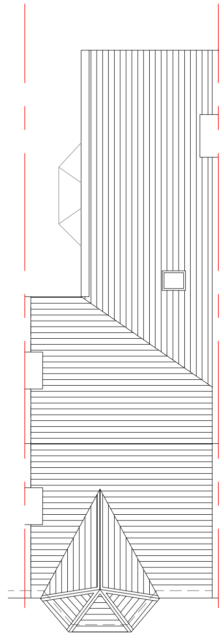
EXISTING ROOF PLAN SCALE 1:100
