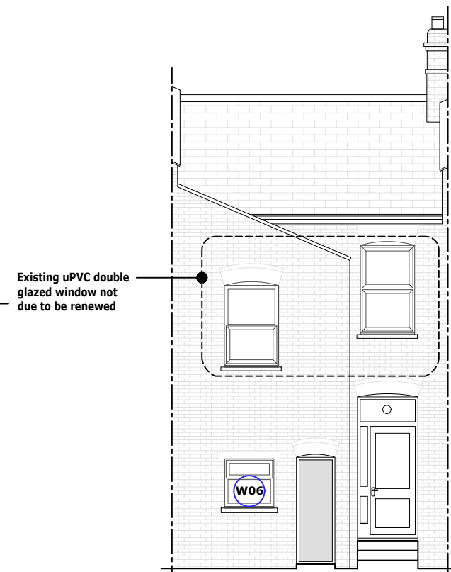
3 Existing West Elevation
