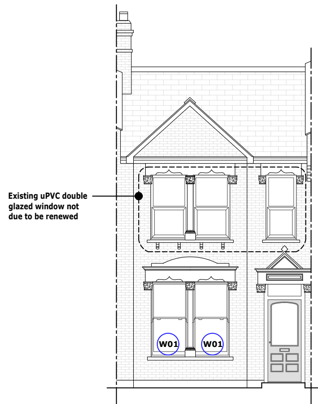
1 Existing East Elevation
