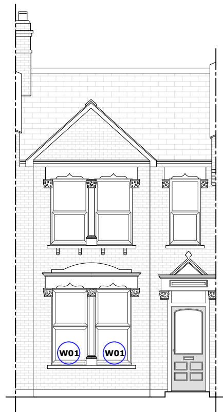
4 Proposed East Elevation
