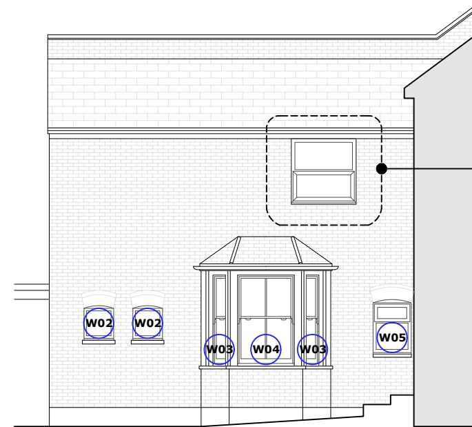
2 Existing South Elevation
