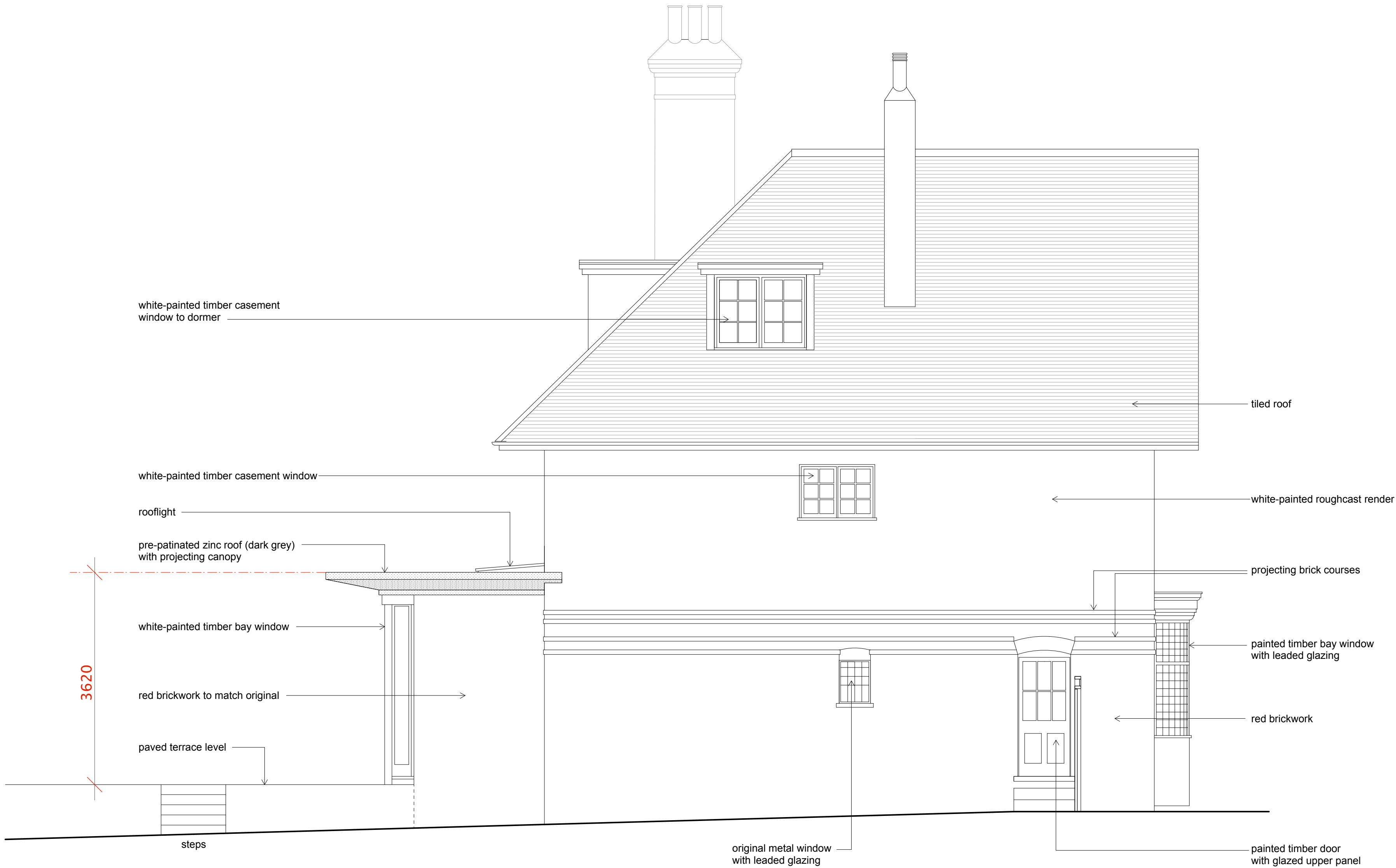
SIDE ELEVATION AS PROPOSED
