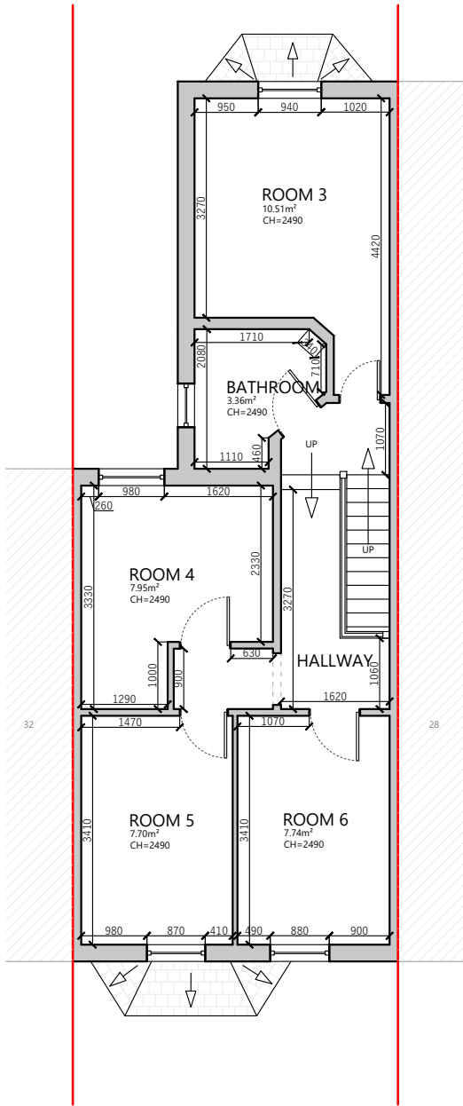
B EXISTING FIRST FLOOR PLAN
