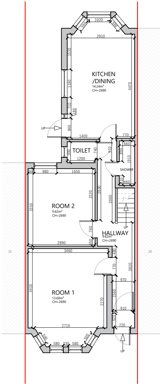
A EXISTING GROUND FLOOR PLAN
