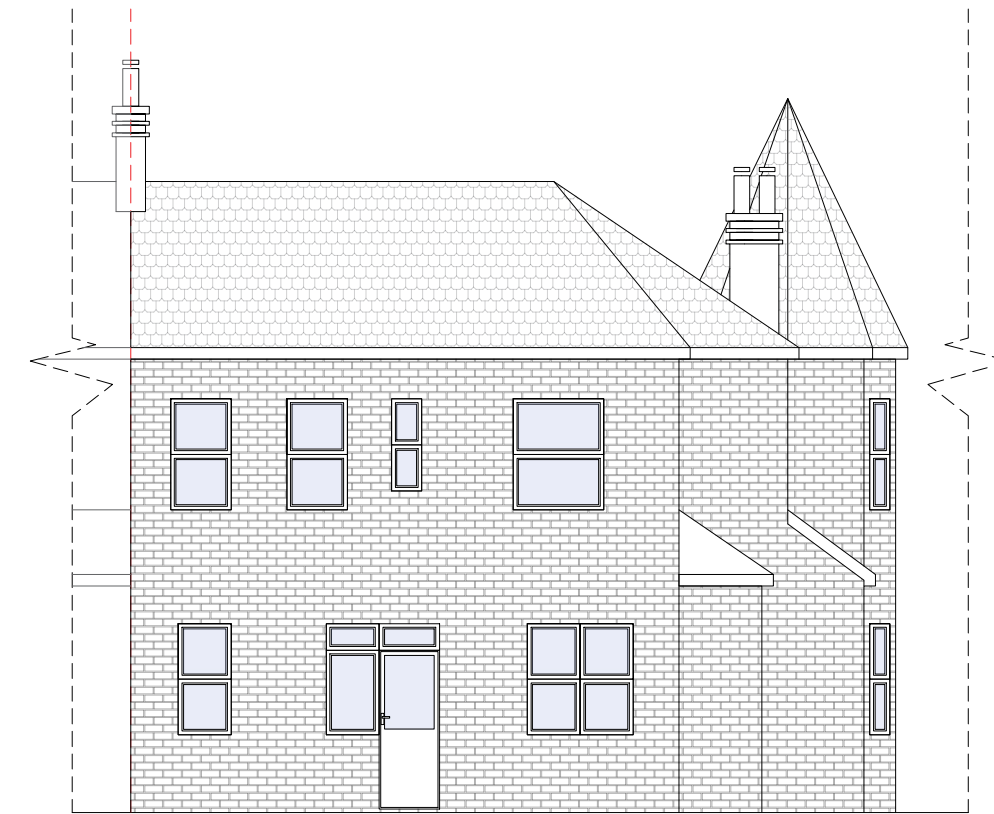
Pre-Existing South Elevation
