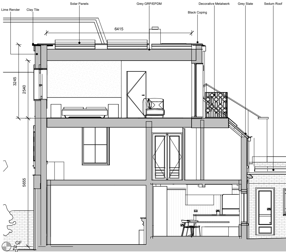
1 PROPOSED LONG SECTION . 1 : 50
