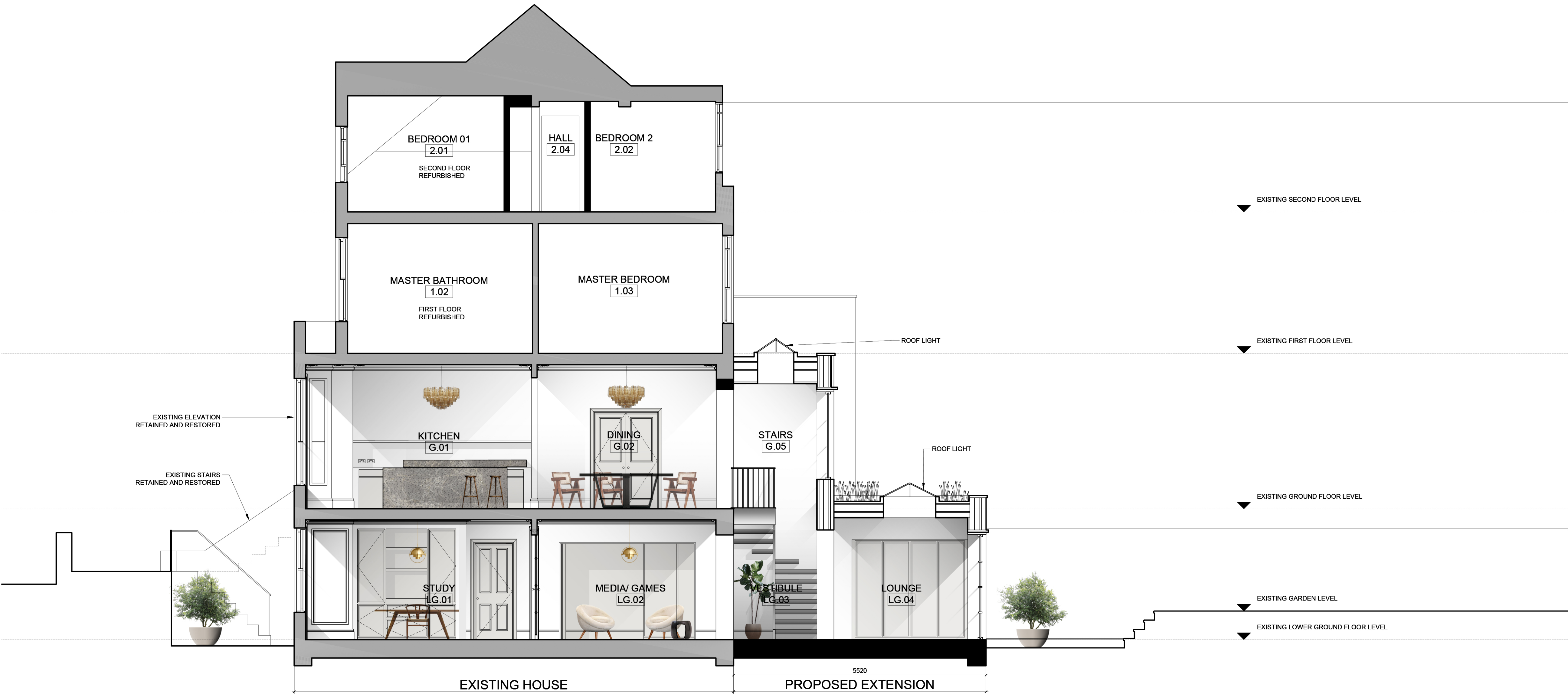
A | PROPOSED SECTION Scale: 1:50 | SECTION
