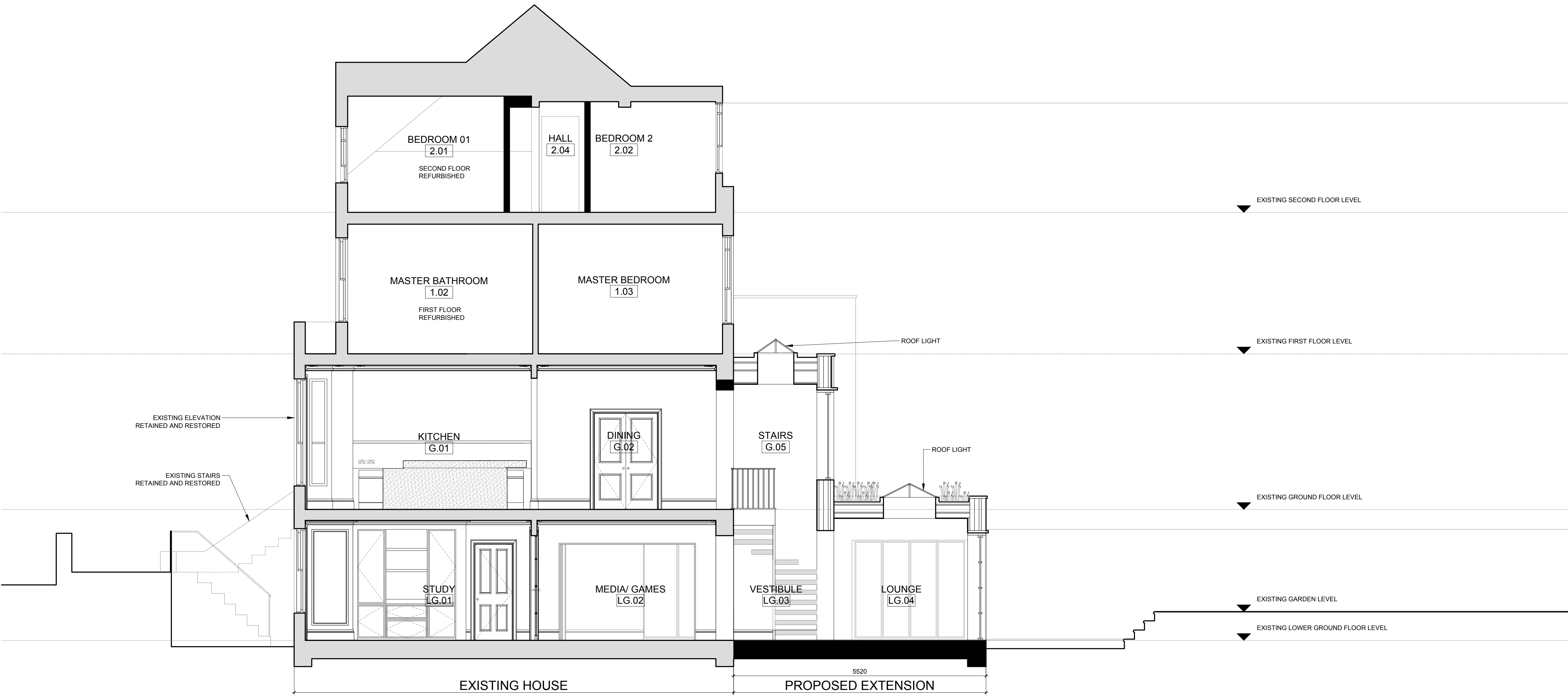
A | PROPOSED SECTION Scale: 1:50 | SECTION 0 1 2 3 4 5 10m
