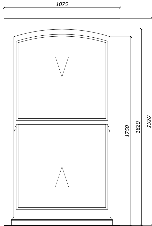
W-5 1 st FLOOR FRONT WINDOW 24mm GLAZING / 4mm / 16mm / 4mm
