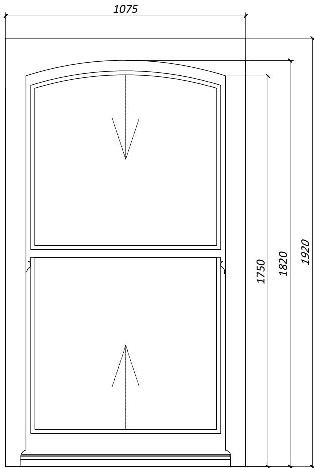
W-4 1 st FLOOR FRONT WINDOW 24mm GLAZING / 4mm / 16mm / 4mm
