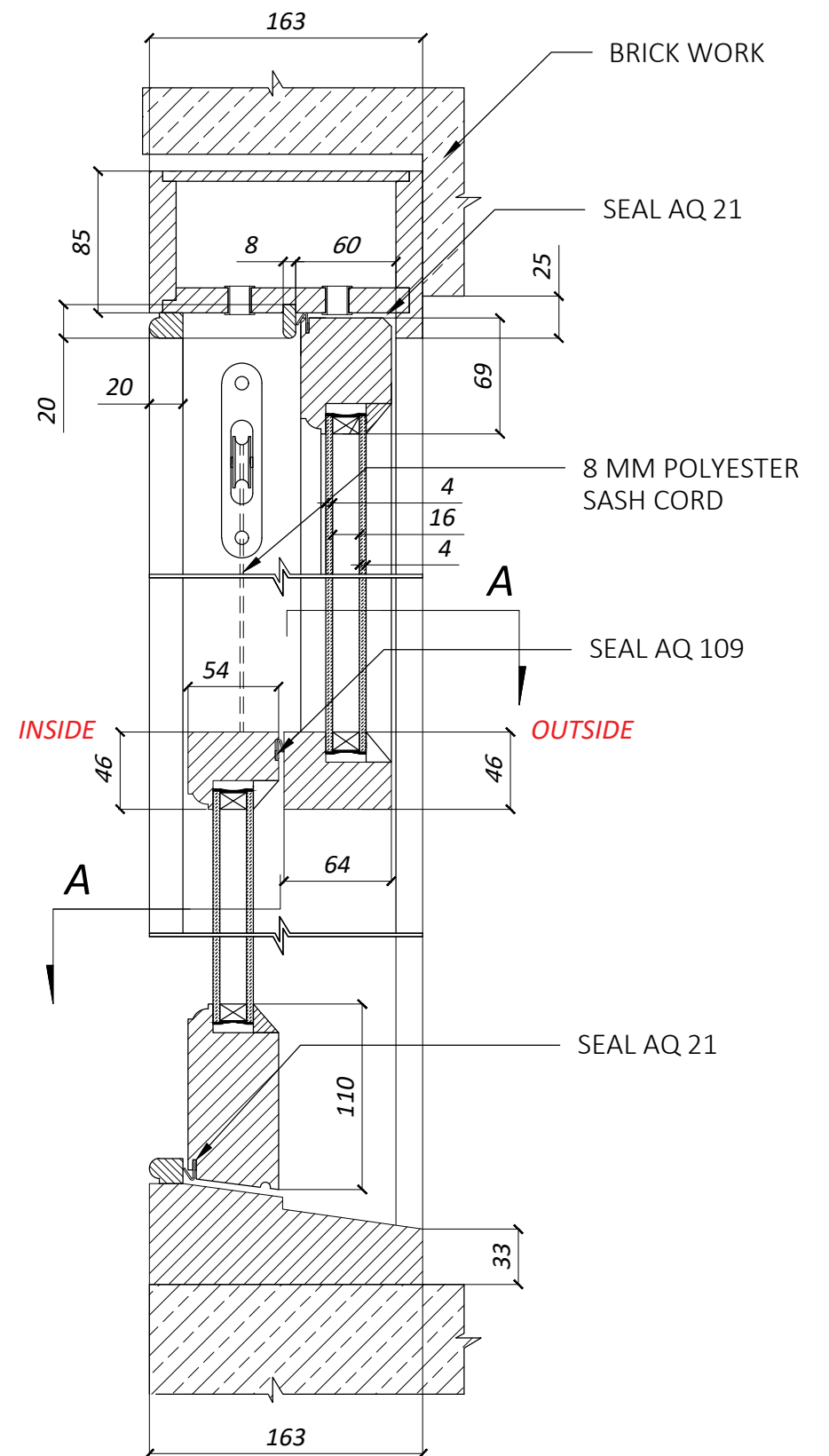
DETAIL 1 / 24 mm GLAZING SCALE 1:4
