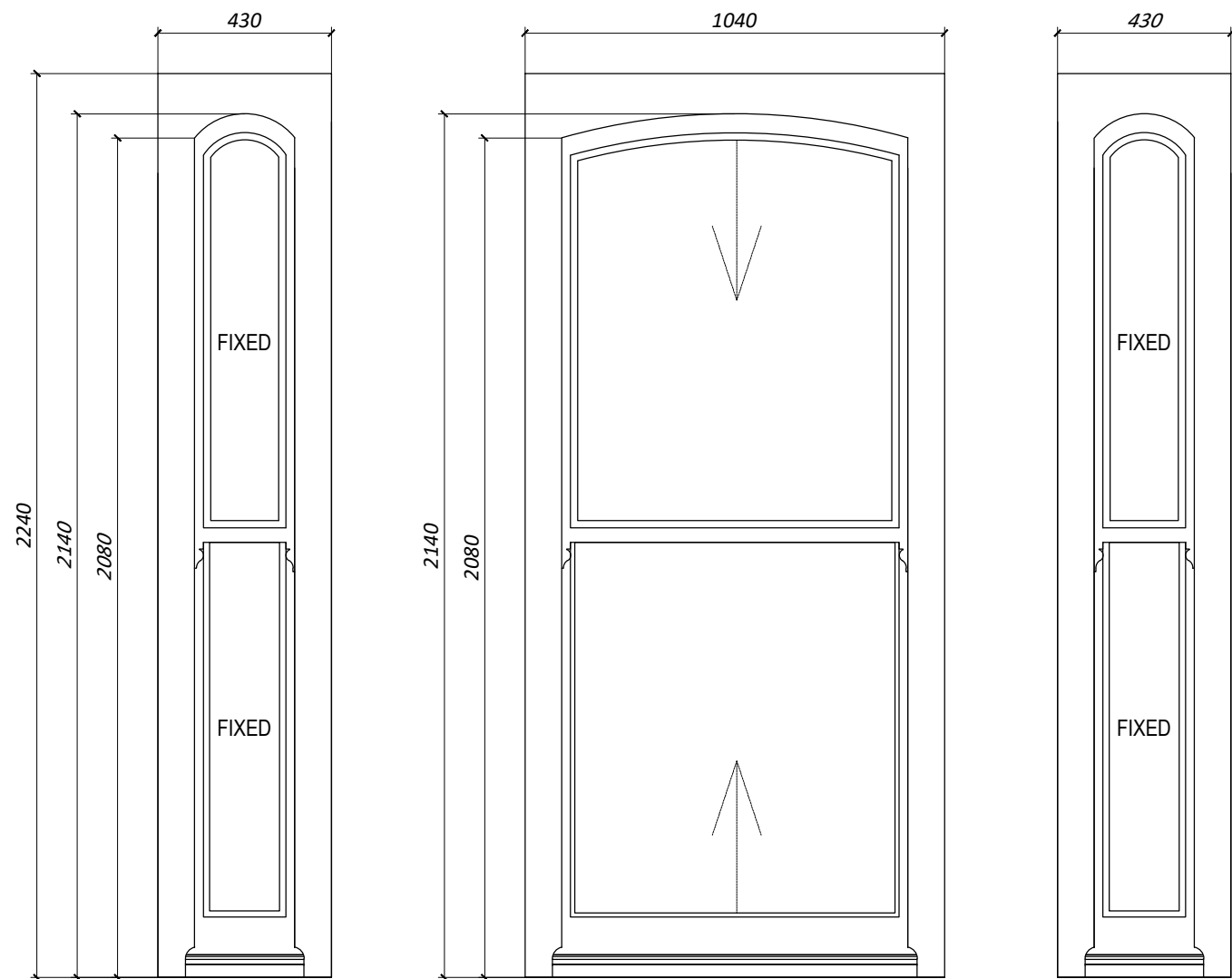
W-1 W-2 W-3 GROUNDFLOOR FRONT BAY WINDOWS 24mm GLAZING / 4mm /16mm /4mm
