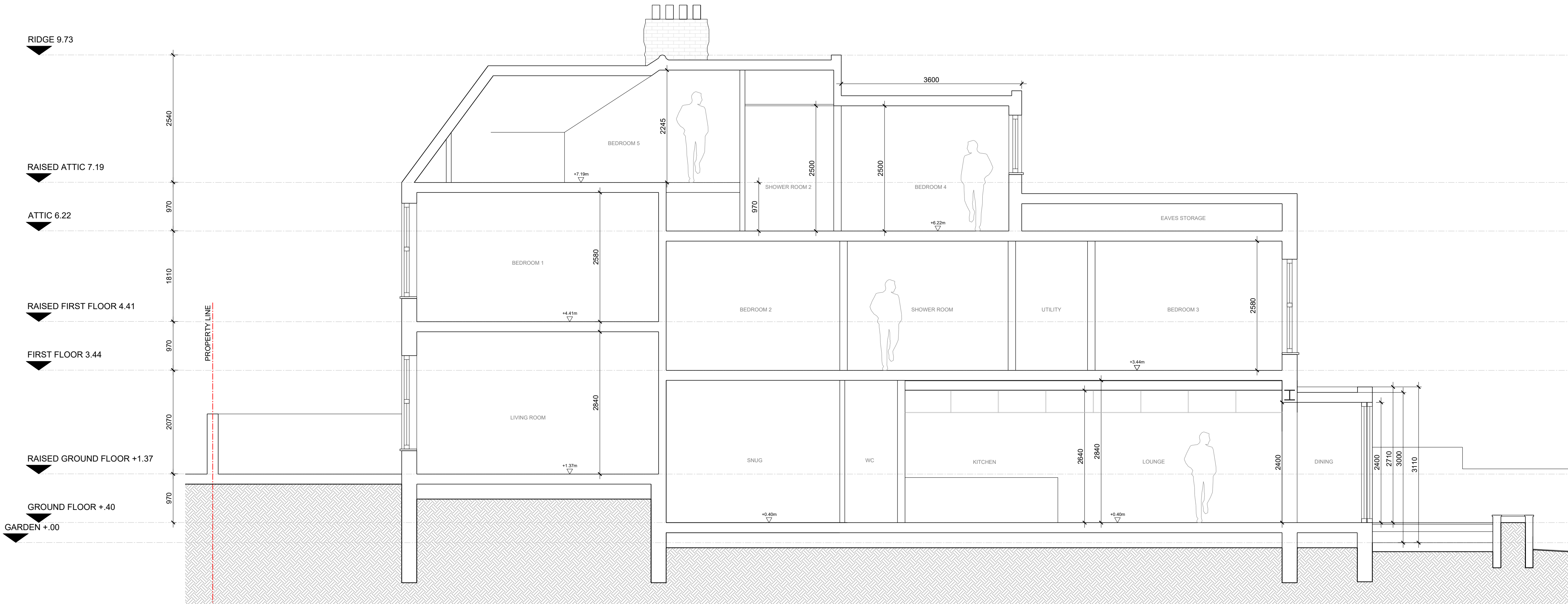
2 PROPOSED SECTION 1 : 50
