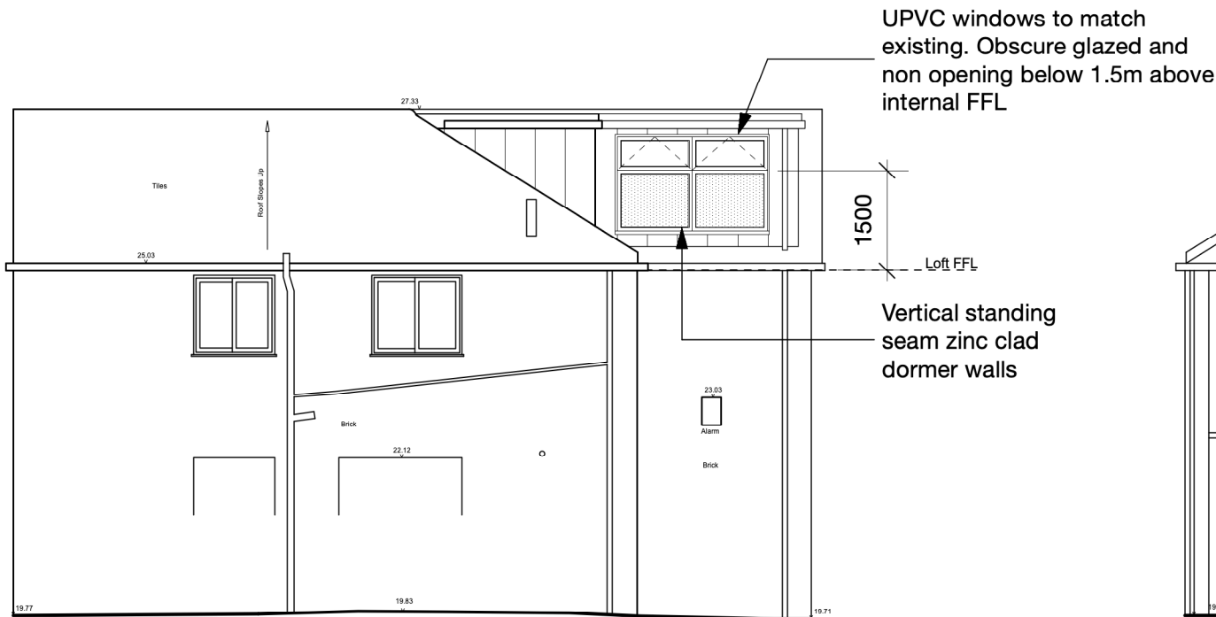
South Elevation 3
