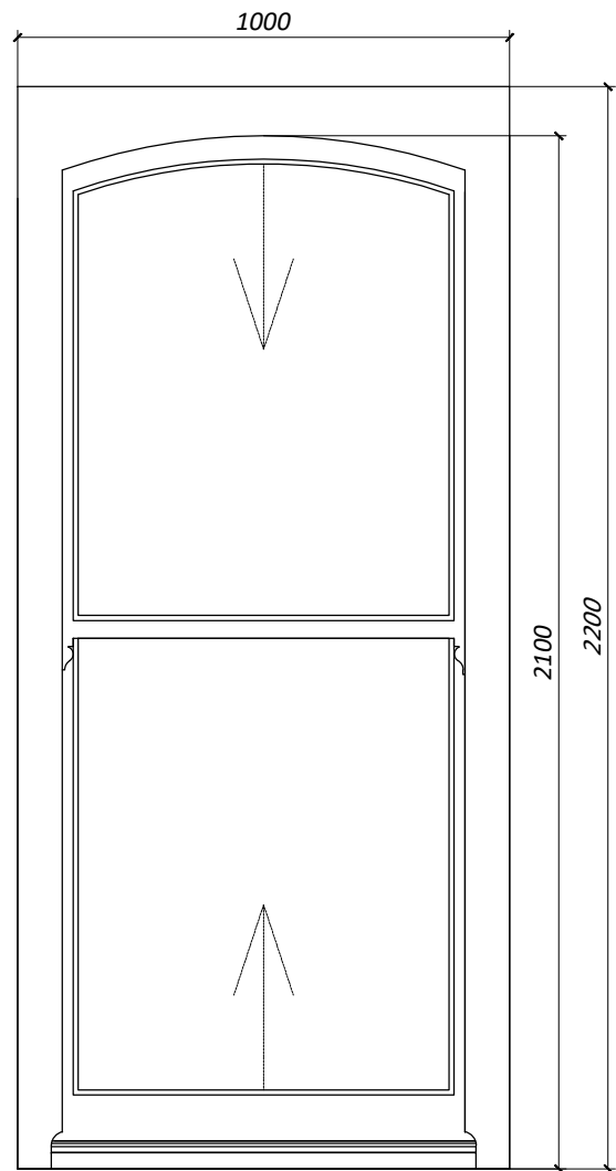
W-03 277_FLAT B FRONT WINDOW SLIMLINE / 14mm GLAZING / 4mm/6mm/4mm
