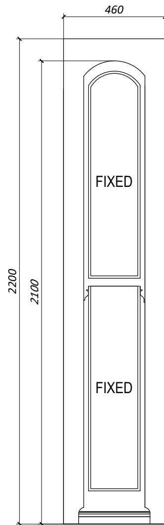
W-04 277_FLAT B FRONT WINDOW BAY SLIMLINE / 14mm GLAZING / 4mm/6mm/4mm
