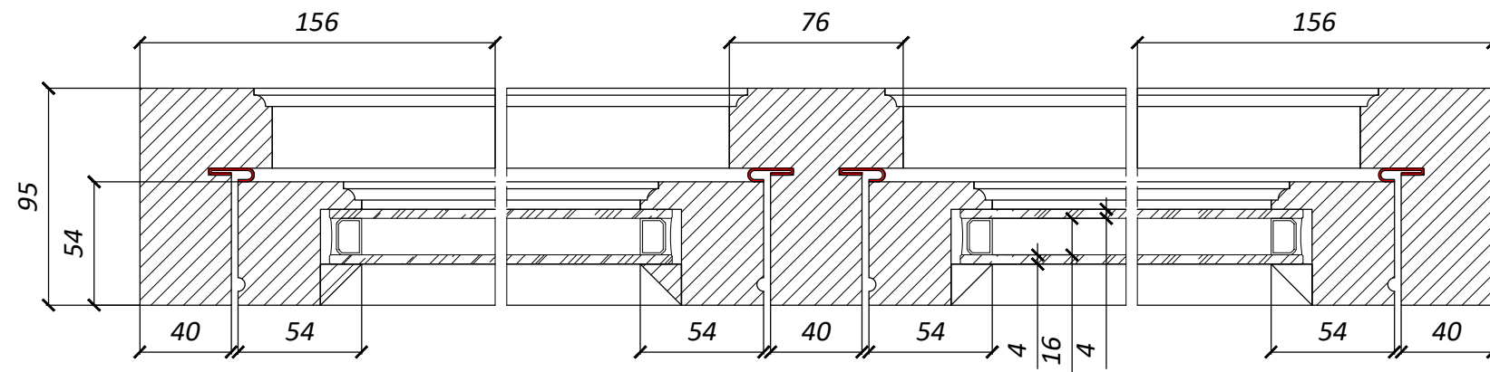
DETAIL 1 / 24 mm GLAZING SCALE 1:3
