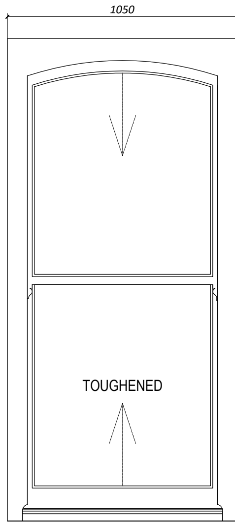
W-04 277_FLAT B FRONT WINDOW BAY SLIMLINE / 14mm GLAZING / 4mm/6mm/4mm
