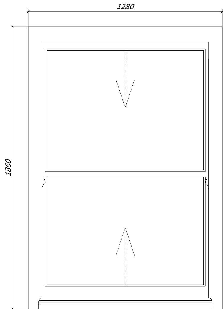
W-09 279_FLAT C / KITCHEN / BACK 24mm GLAZING / 4mm / 16mm / 4mm
