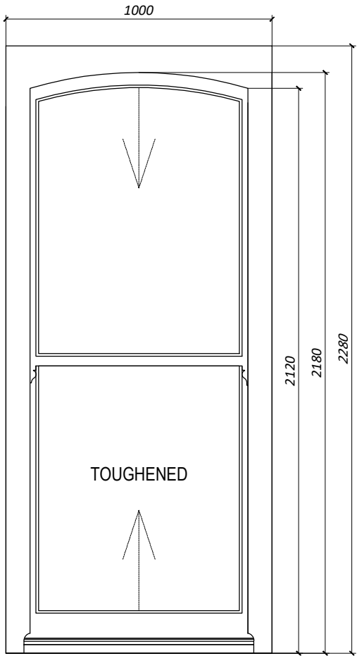
W-03 279_FLAT B FRONT WINDOW SLIMLINE / 14mm GLAZING / 4mm/6mm/4mm
