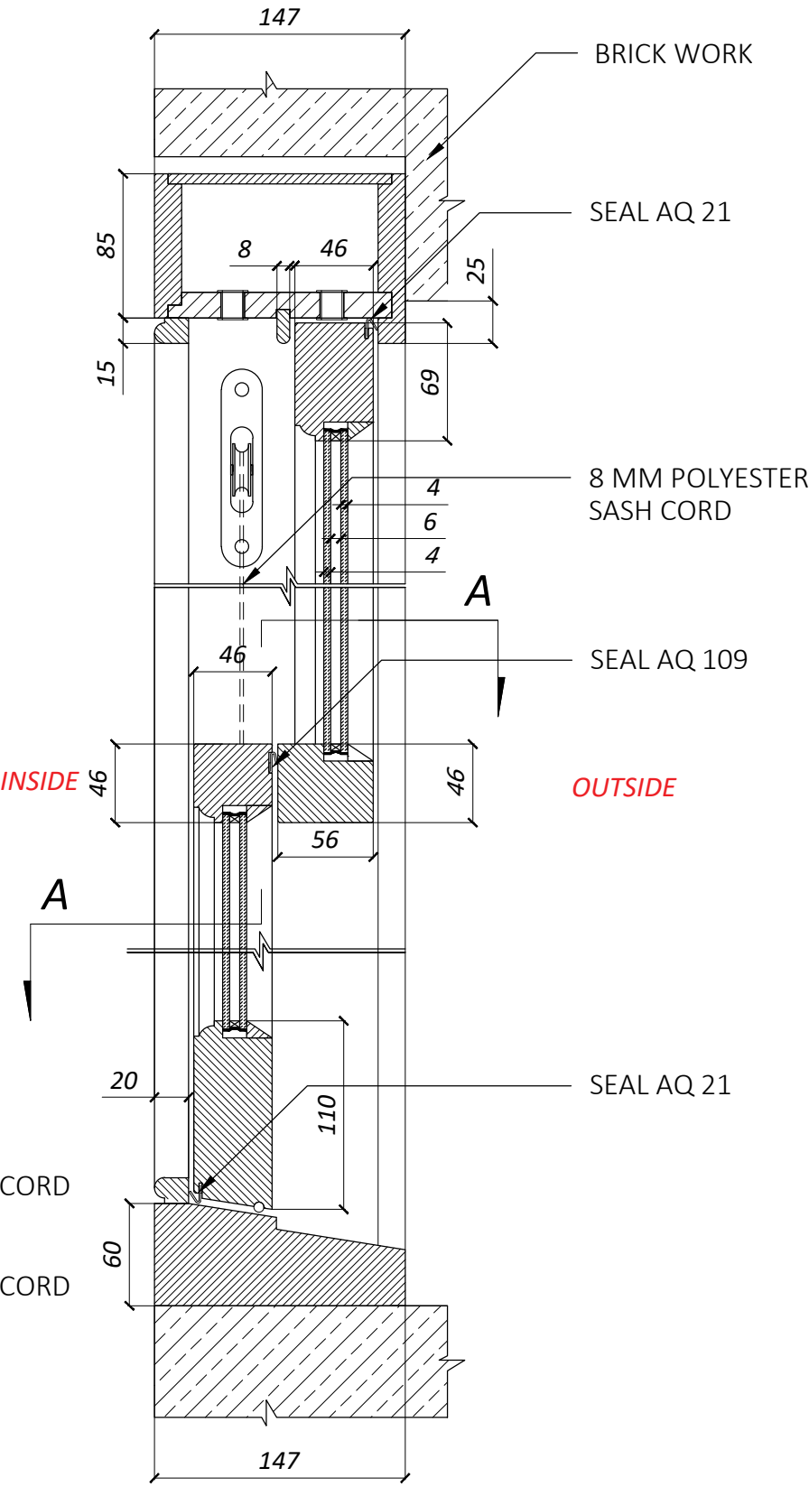
DETAIL 1 / 14 mm GLAZING SCALE 1:4
