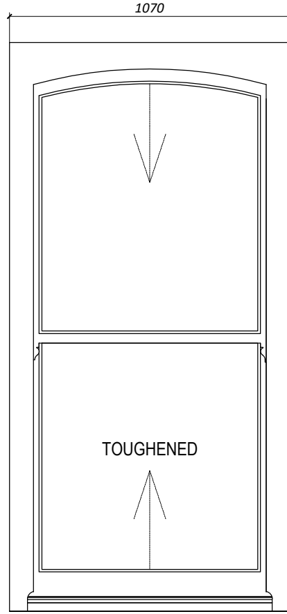
W-04 279_FLAT B FRONT WINDOW BAY SLIMLINE / 14mm GLAZING / 4mm/6mm/4mm
