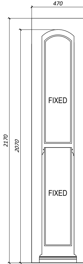
W-04 279_FLAT B FRONT WINDOW BAY SLIMLINE / 14mm GLAZING / 4mm/6mm/4mm
