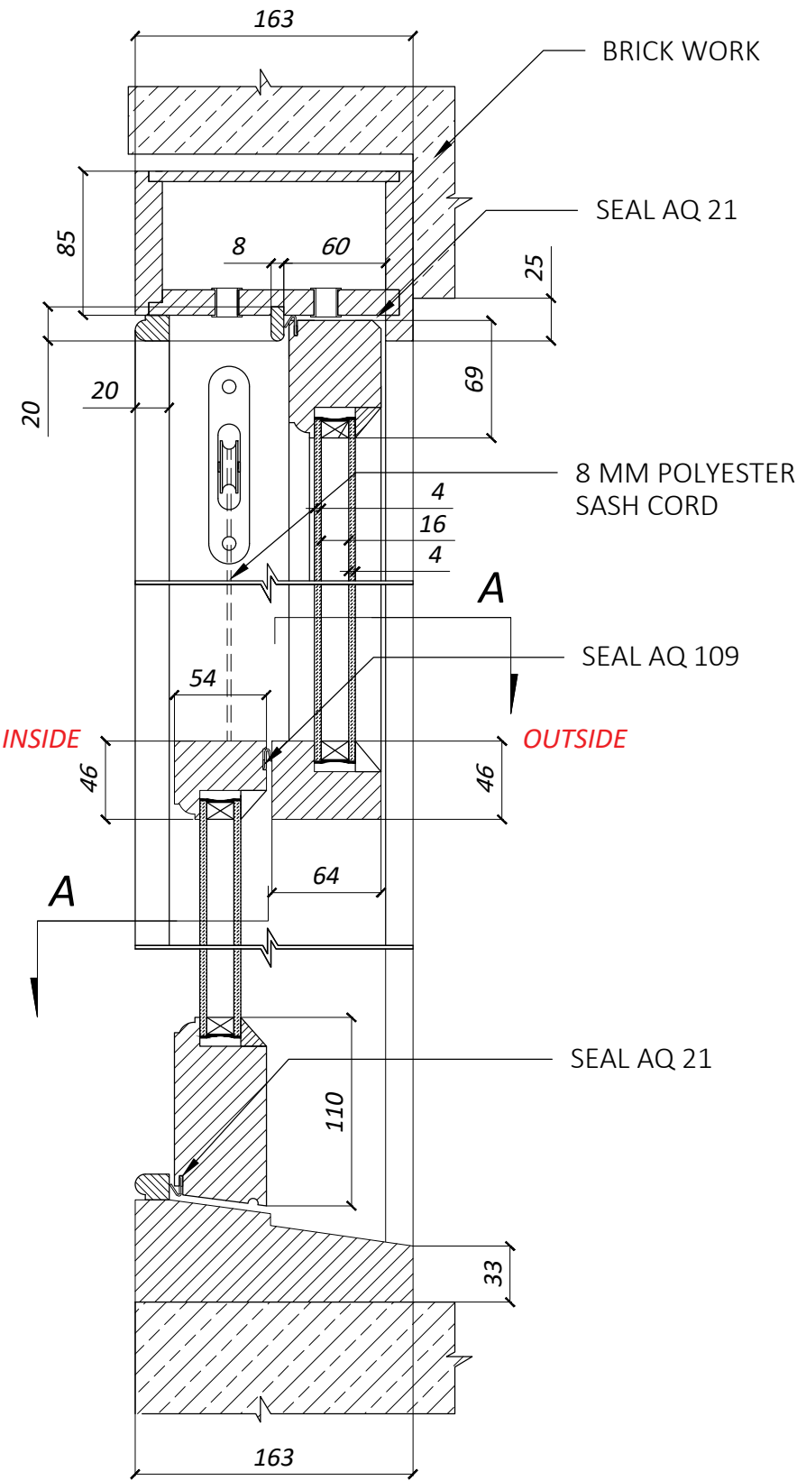
DETAIL 1 / 24 mm GLAZING SCALE 1:4
