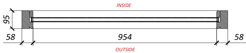
PLAN A GLAZING 24mm / 4mm / 16mm / 4mm
