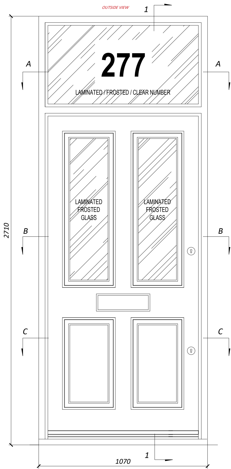
PLAN A GLAZING 24mm / 4mm / 16mm / 4mm
