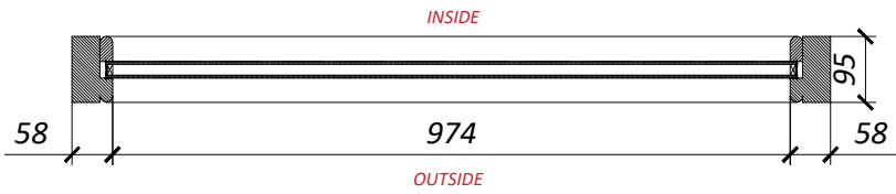
PLAN B GLAZING 24mm / 6,4mm / 12mm / 6,4mm
