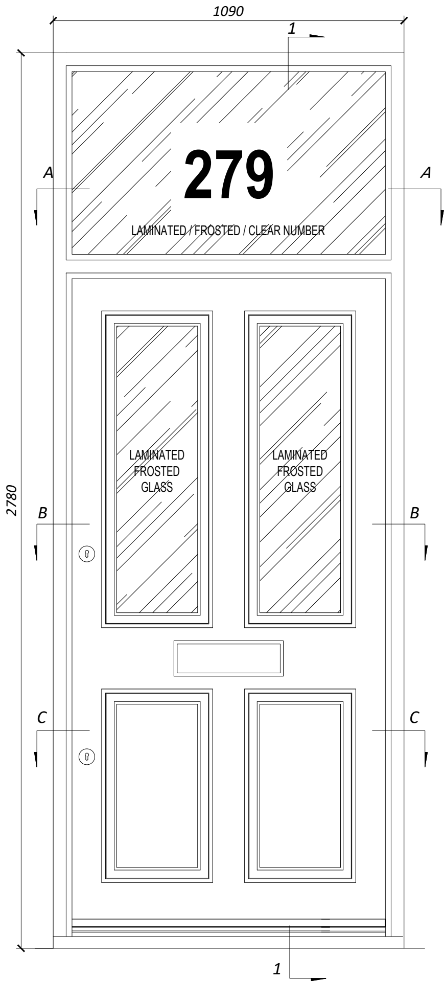
PLAN A GLAZING 24mm / 4mm / 16mm / 4mm
