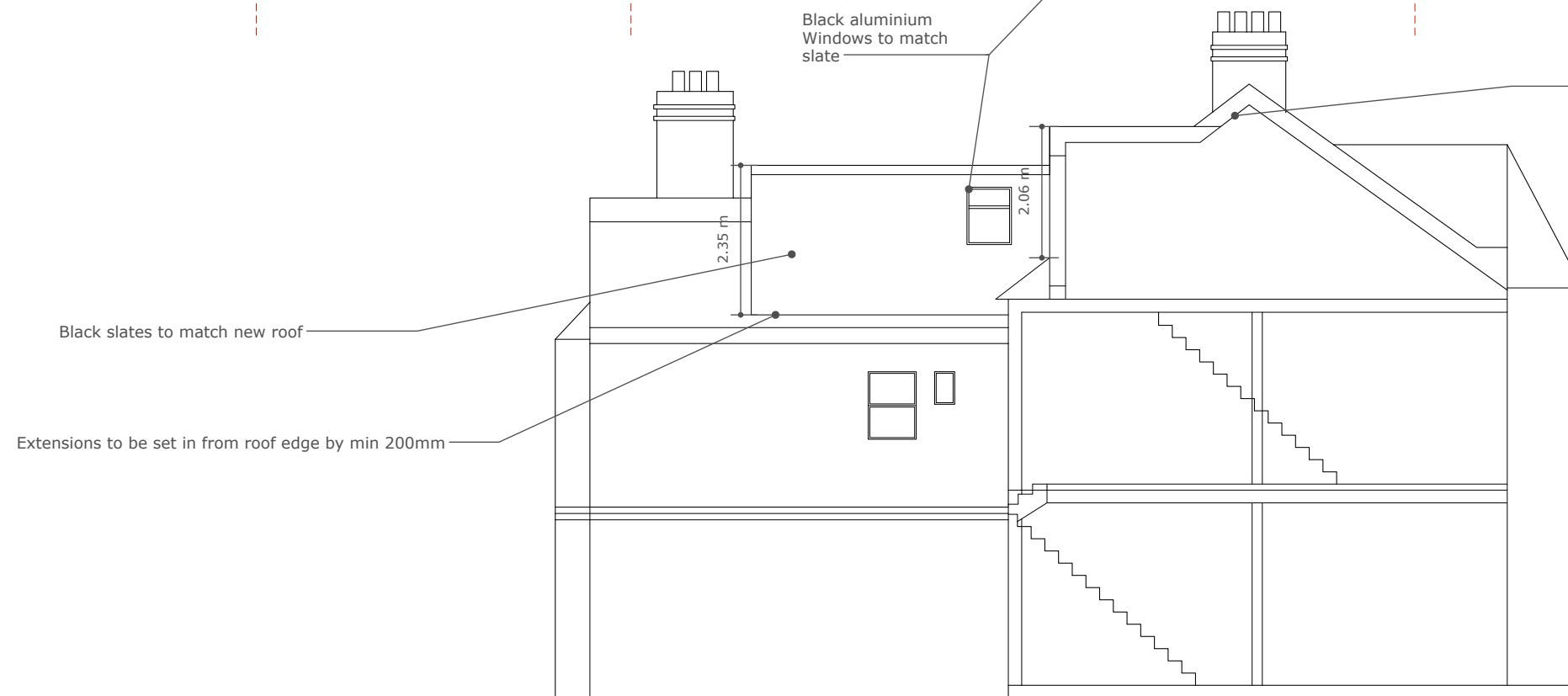
Rear section
