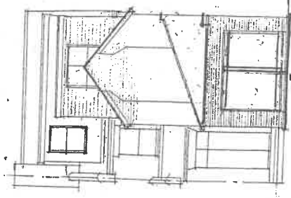
REAR ELEVATION
