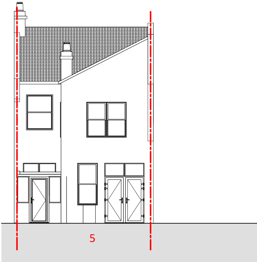
1 EXISTING REAR ELEVATION 1 : 100
