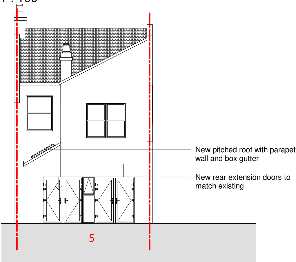
2 PROPOSED REAR ELEVATION 1 : 100
