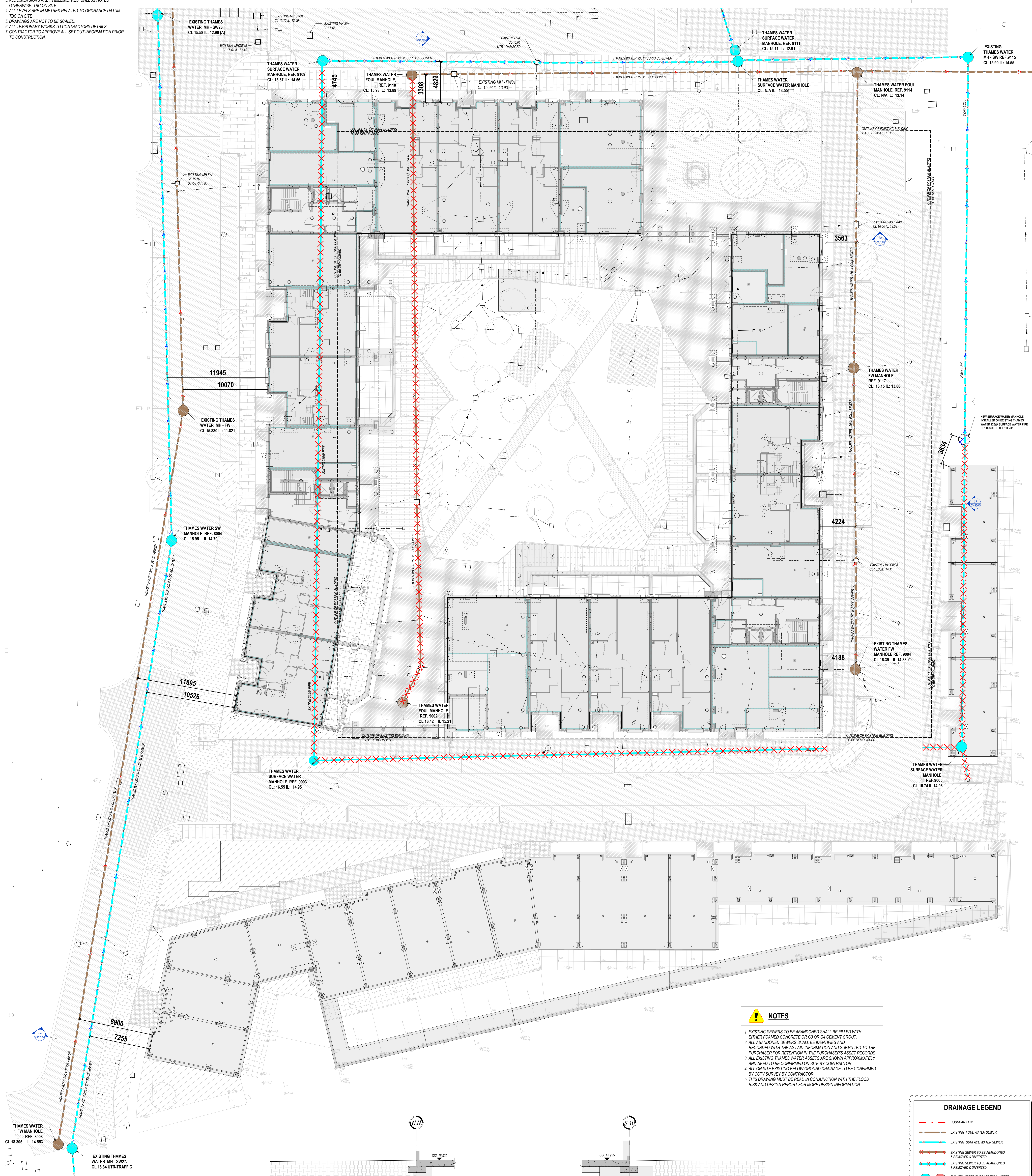
Abandoned Sewer Layout SCALE 1 : 150
