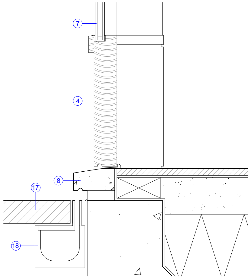
DETAIL 07 1:5@A3
