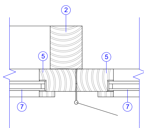
DETAIL 04 1:5@A3
