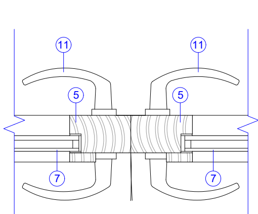
DETAIL 05 1:5@A3
