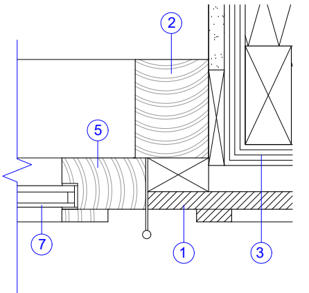
DETAIL 06 1:5@A3
