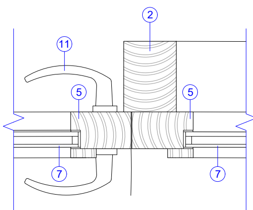
DETAIL 02 1:5@A3
