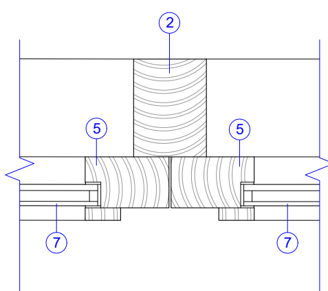
DETAIL 03 1:5@A3
