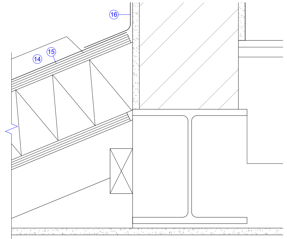
DETAIL 09 1:5@A3
