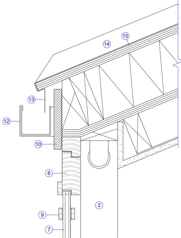
DETAIL 08 1:5@A3
