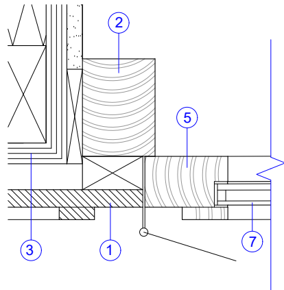
DETAIL 01 1:5@A3
