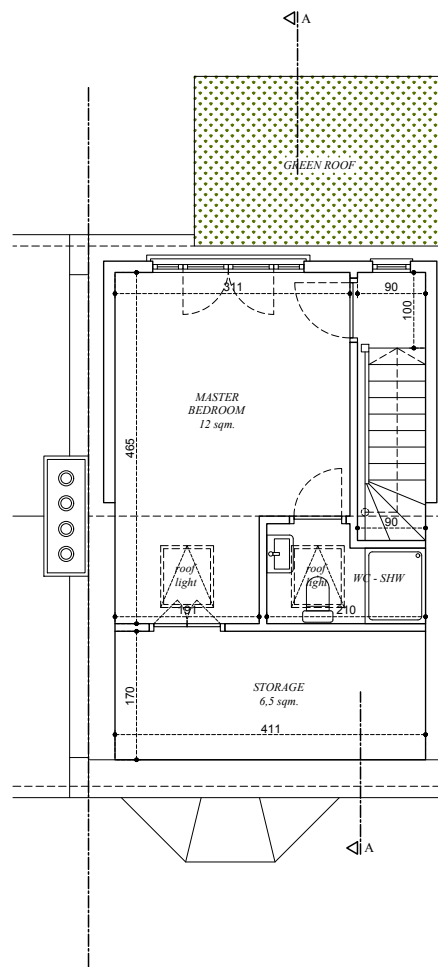
PROPOSED LOFT PLAN
