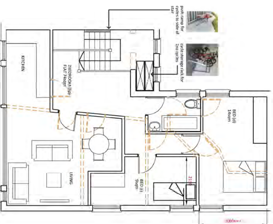
FIRST FLOOR PLAN - PROPOSED
