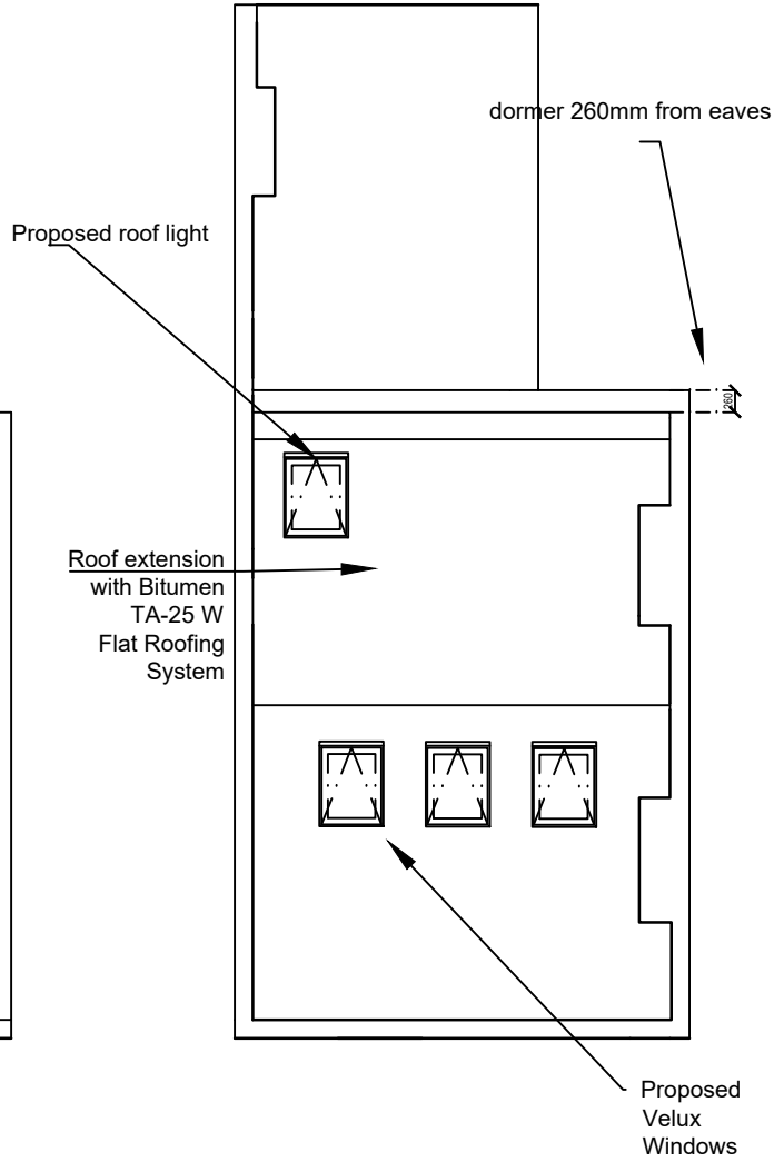
Roof Plan
