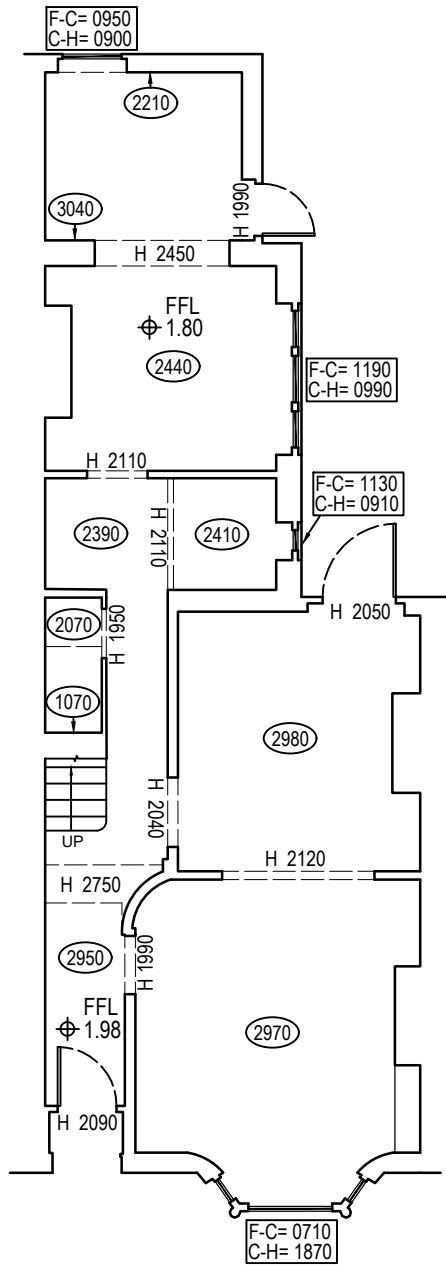
Ground Floor
