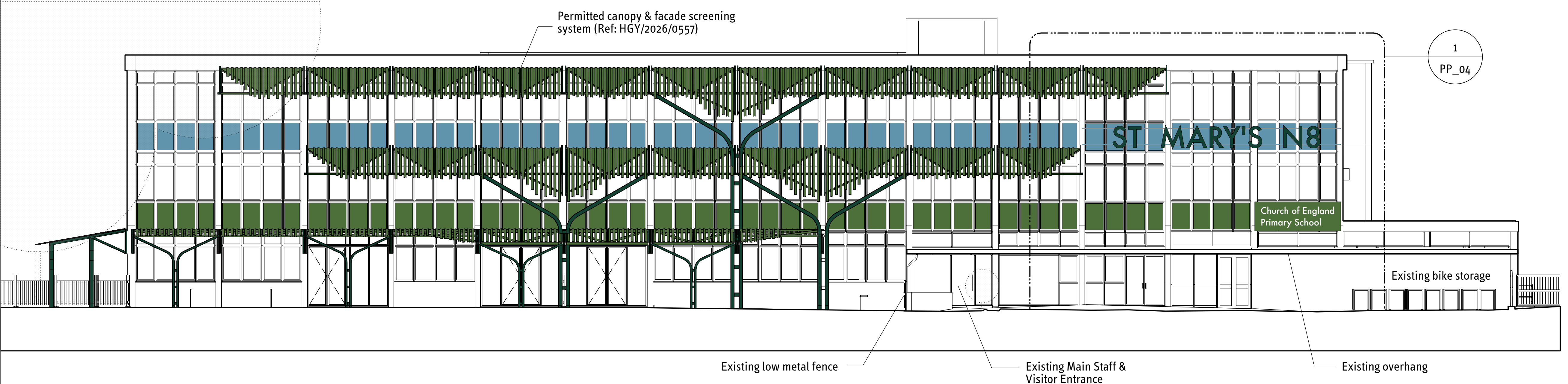
2 PROPOSED SIGNAGE - SOUTH FACADE ELEVATION 1:100@A1/1:200@A3
