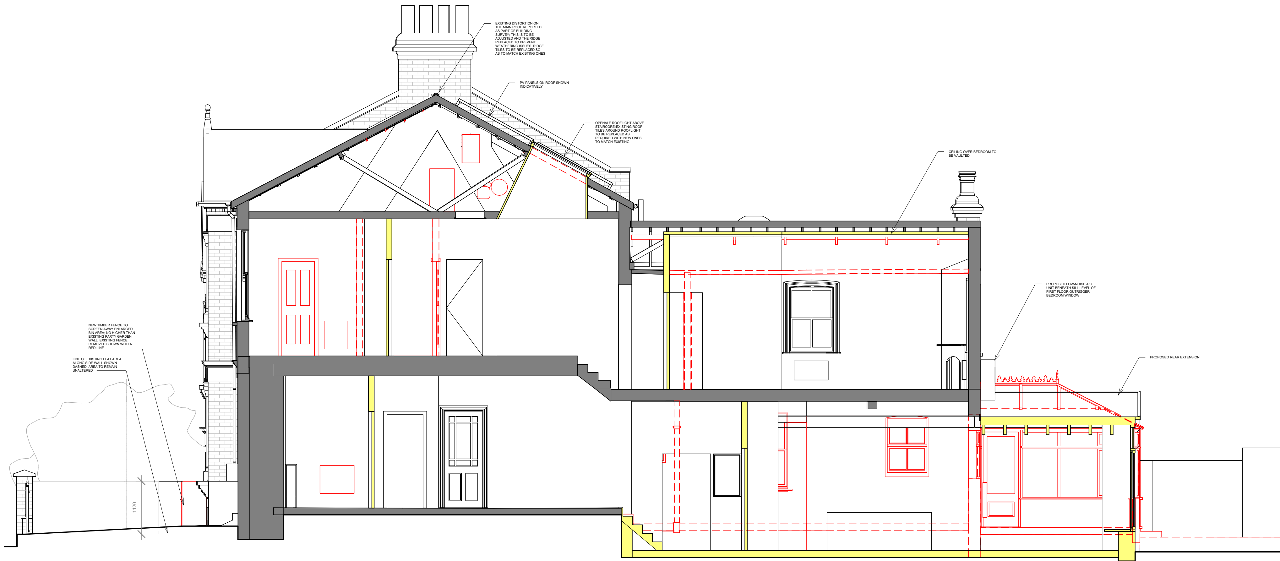
1-PL_2101 PROPOSED LONG SECTION THROUGH DORMERS
