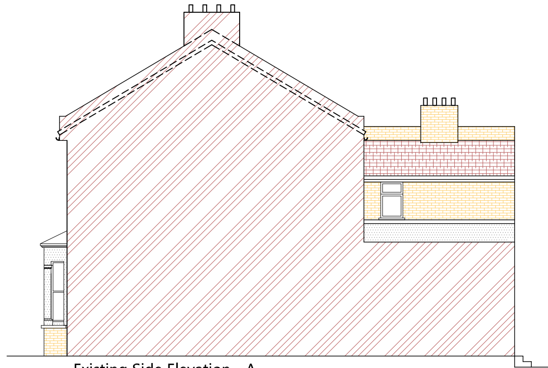
Existing Side Elevation - A
