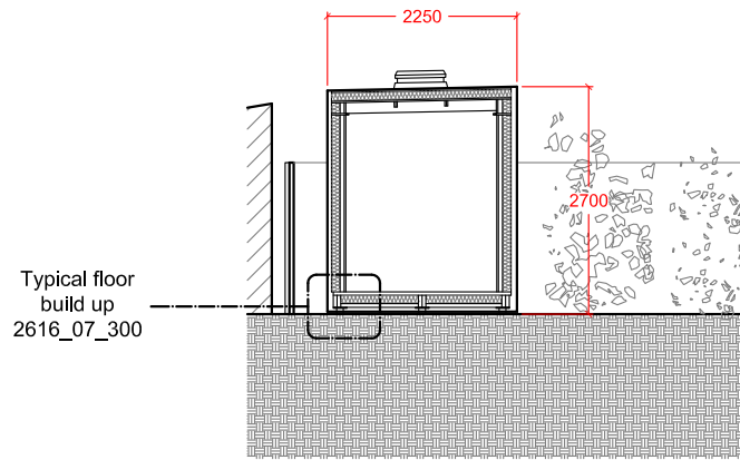
5. PROPOSED SECTION - scale 1:100
