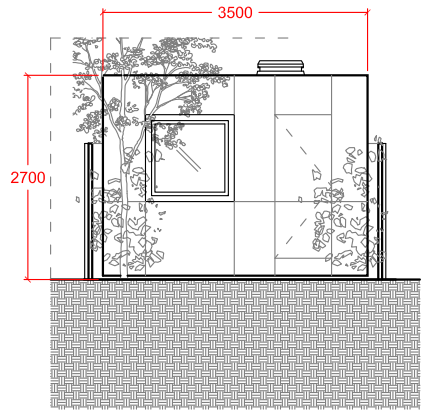
1. PROPOSED FRONT ELEVATION - scale 1:100
