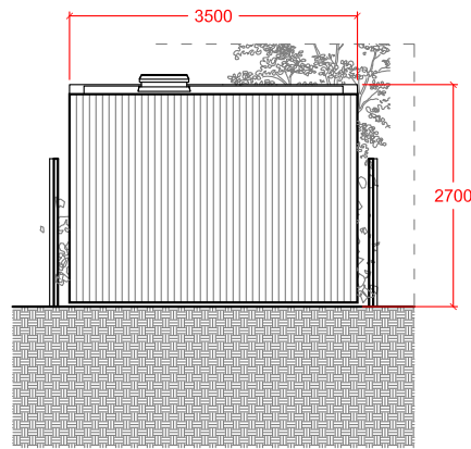
2. PROPOSED REAR ELEVATION - scale 1:100
