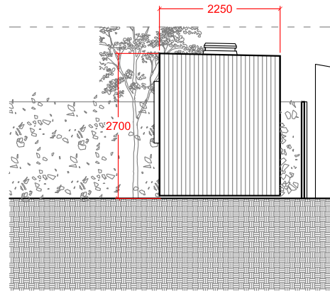
3. PROPOSED RIGHT ELEVATION - scale 1:100
