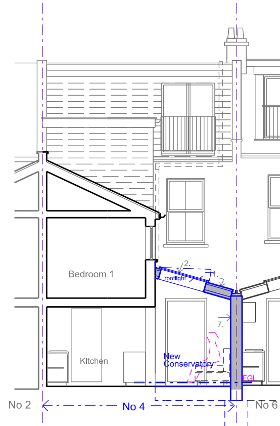
Proposed Section BB Scale 1:100 @ A3
