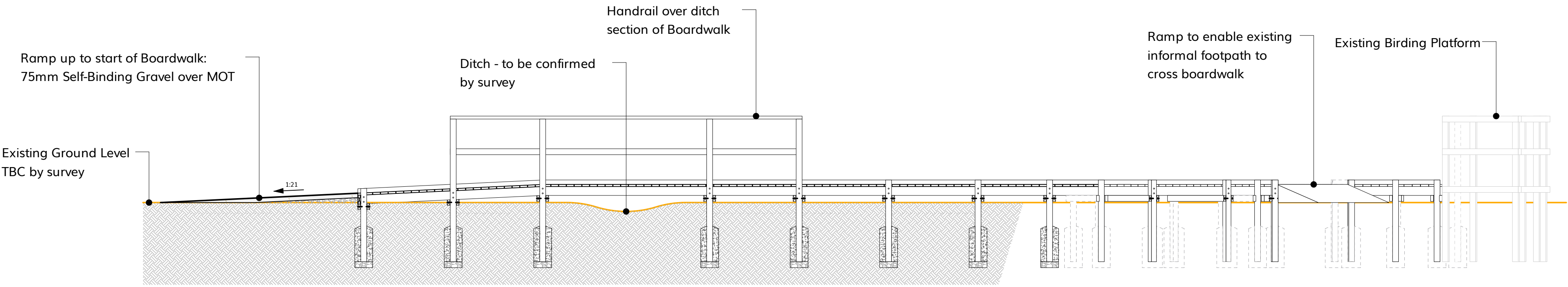
D02 Boardwalk - Indicative Elevation 0502 Scale: 1:50
