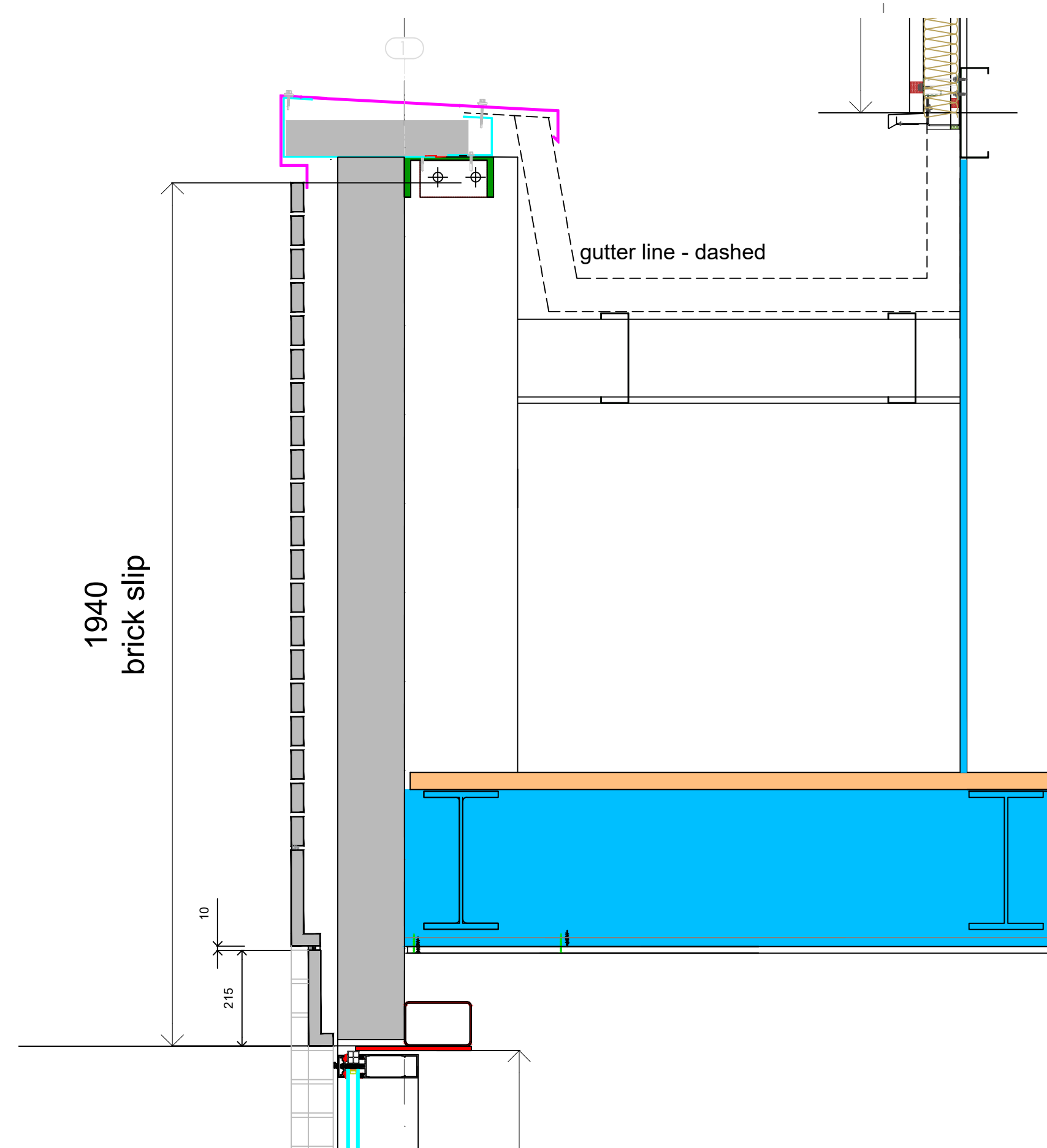
SECTION: D_202 / 2; scale: 1/10
