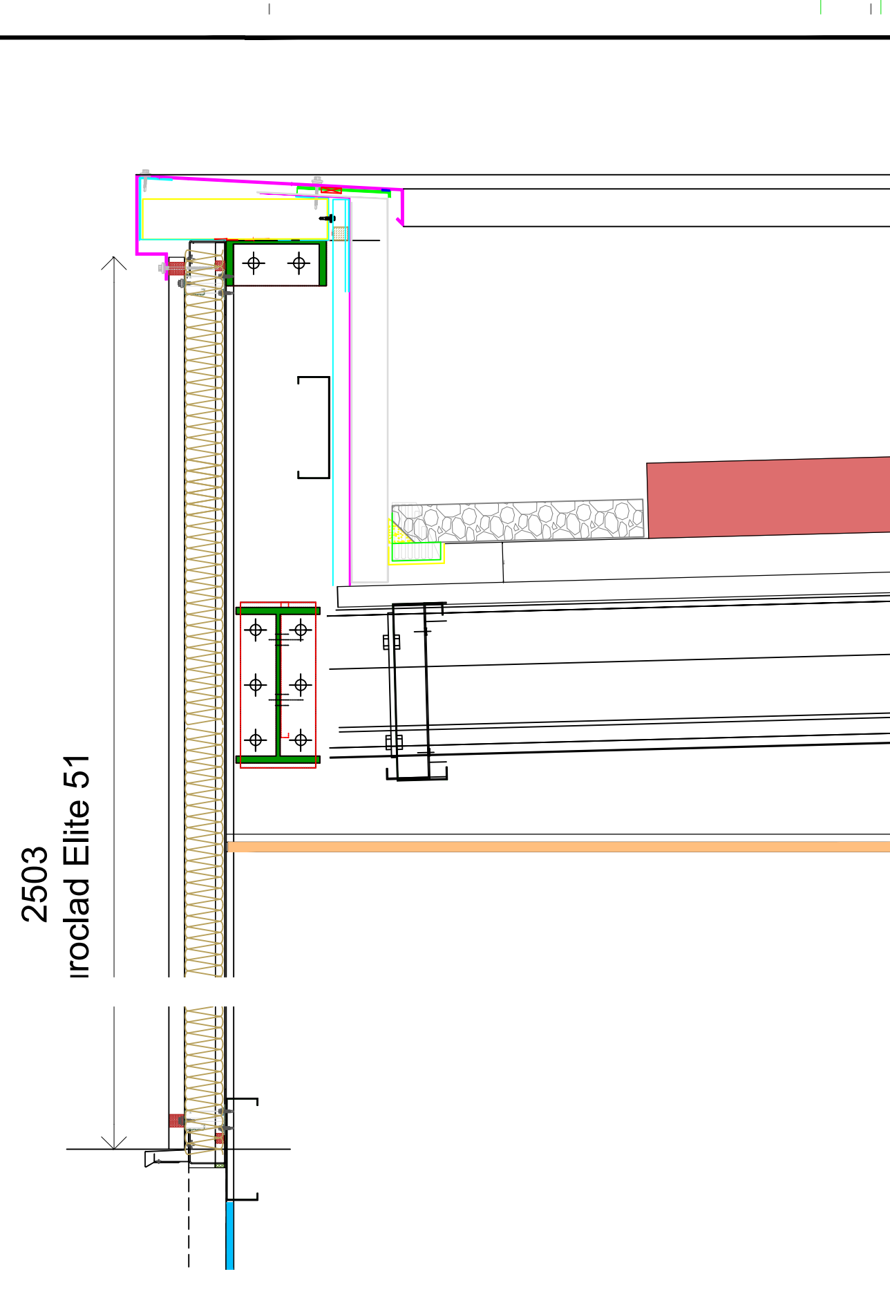
SECTION: D_202 / 3; scale: 1/10
