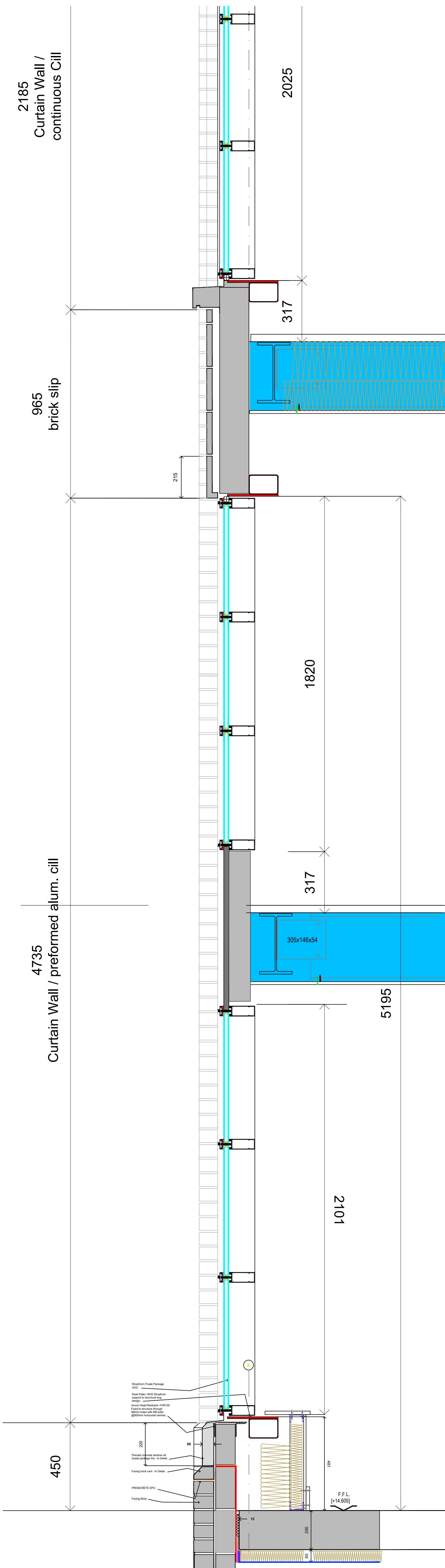
SECTION: D_202 / 1; scale: 1/10
