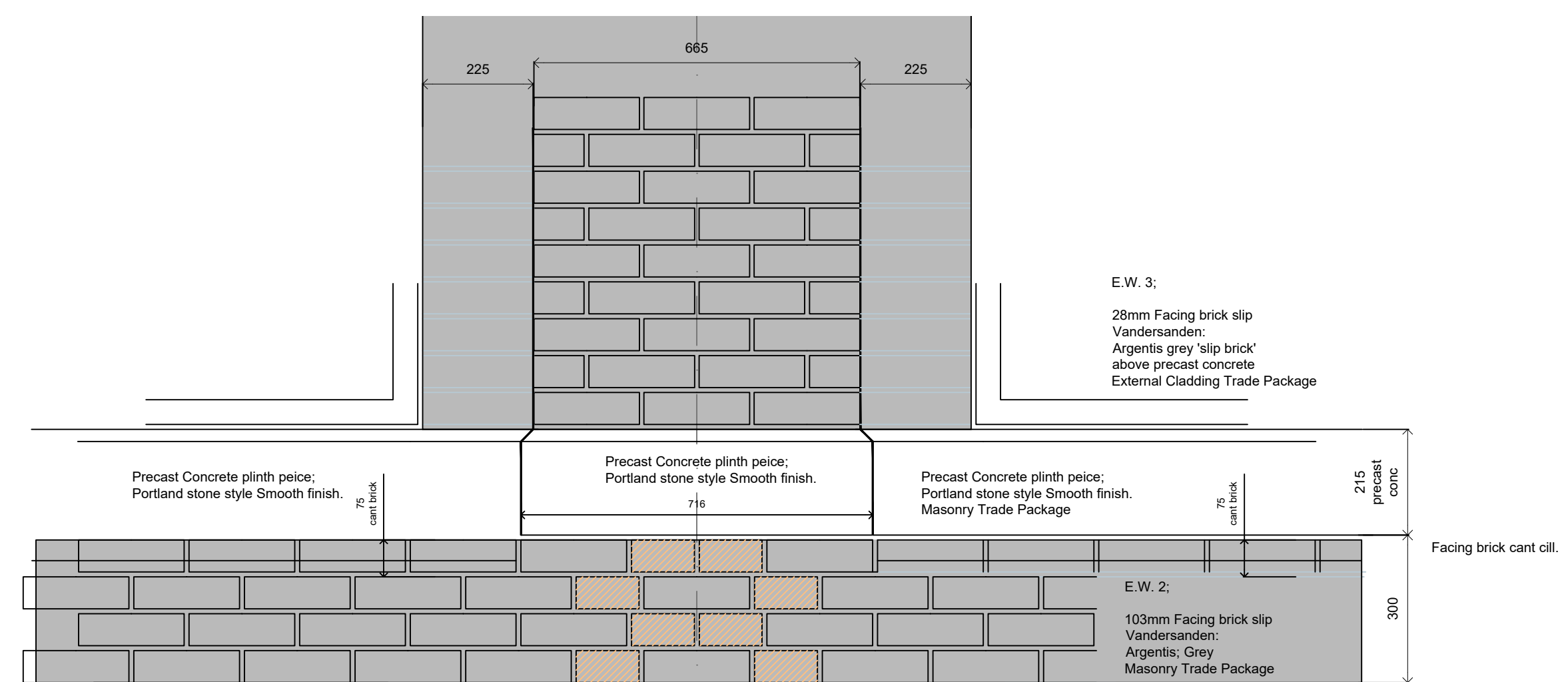
DETAIL: D_203/1; Plinth / Stallriser - scale 1/10
