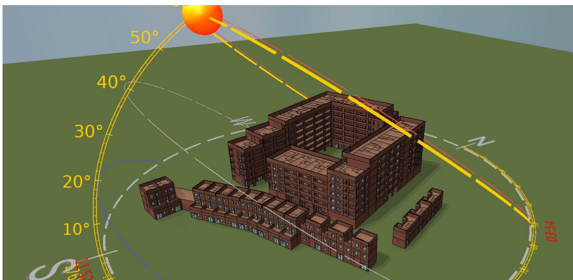
Figure 3: 3D model of the proposed building
