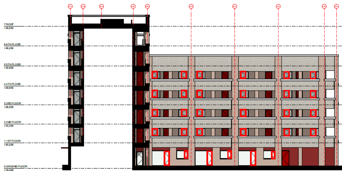
Figure 12: North Facing Elevation – Courtyard – Block A & B
