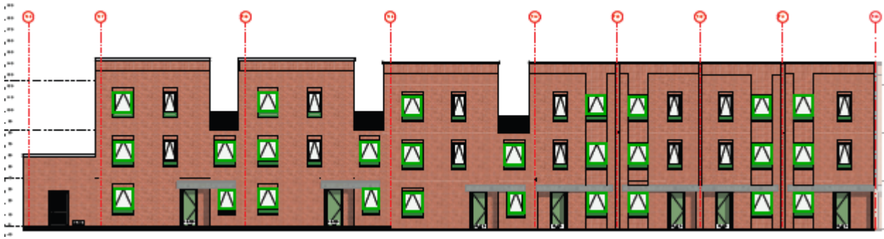
Figure 13: North Elevation 1 – Townhouses
