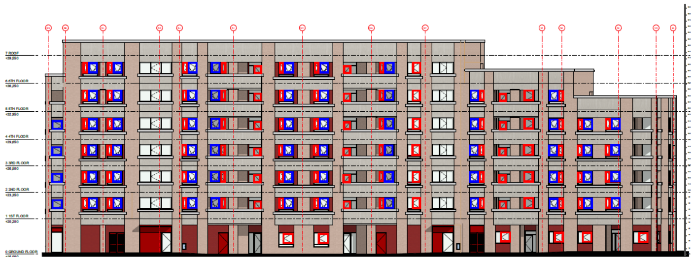
Figure 5: West Elevation - Street – Block A & B
