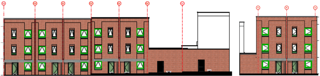
Figure 14: North Elevation 2 – Townhouses
