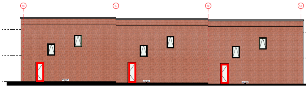
Figure 18: West Elevation 2 – Townhouses
