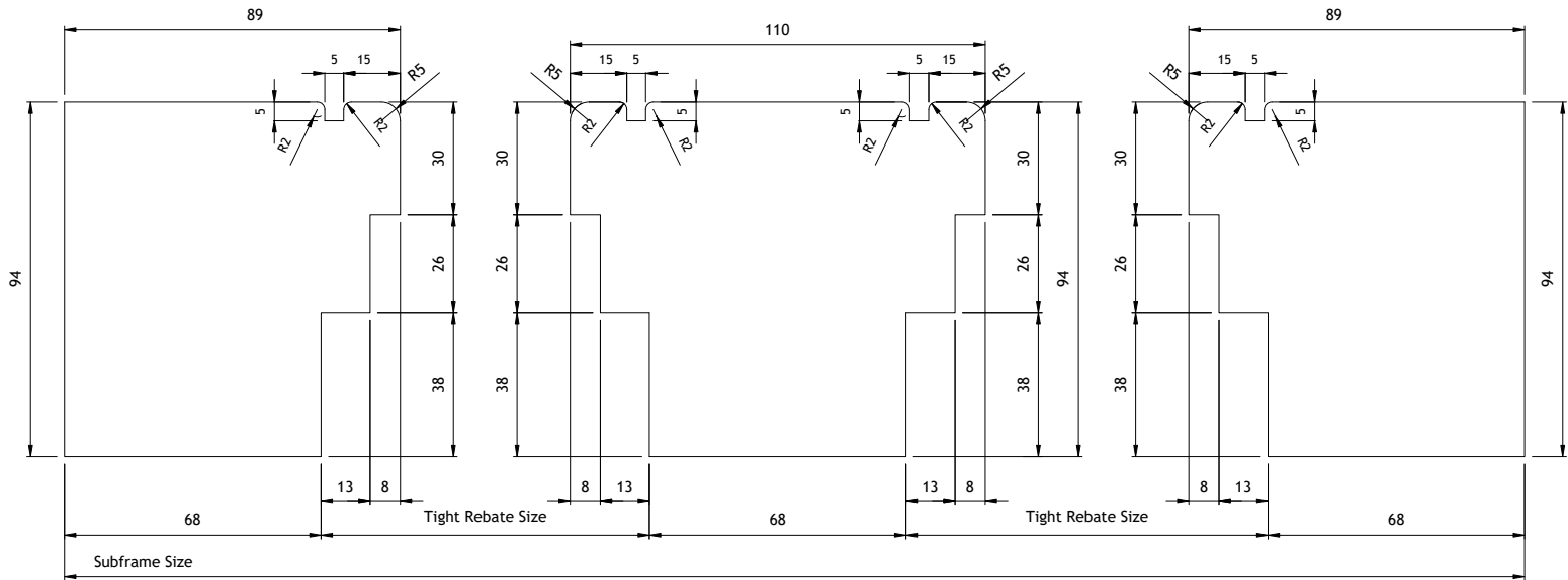
Section TIMA - TIMA
