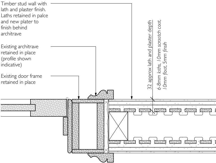
1 Typical Internal Door Architrave Detail Scale: 1:5
