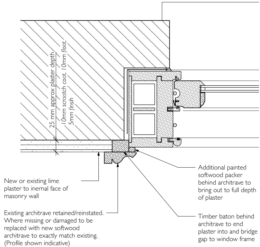
3 Type 2 - Packed Out Window Architrave Plan Detail Scale: 1:5
