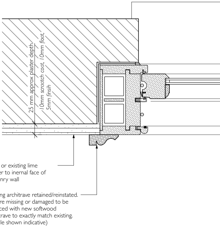
2 Type 1 - Typical Window Architrave Plan Detail Scale: 1:5
