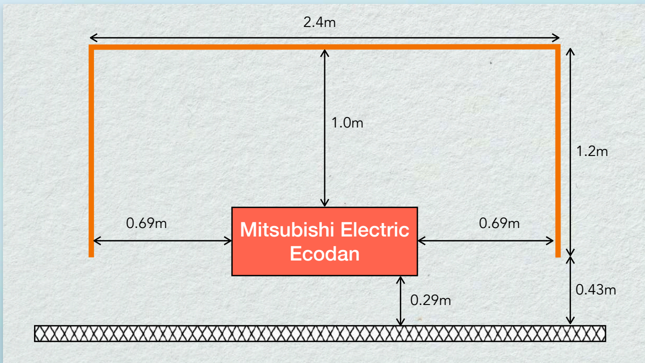
Figure A.3 - ASHP / Noistop original configuration at the outdoor test site, aerial view ( Physical Tests ).
