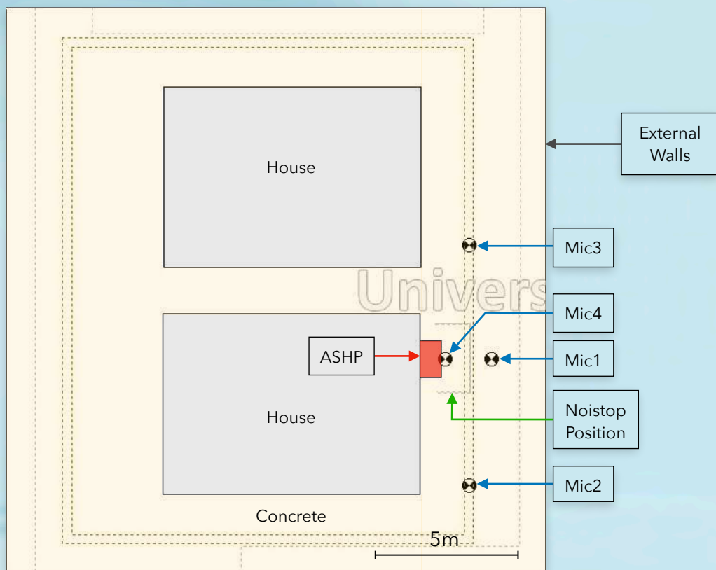
Figure A.2 - Export from CadnaA demonstrating an arial view of the laboratory test location.
