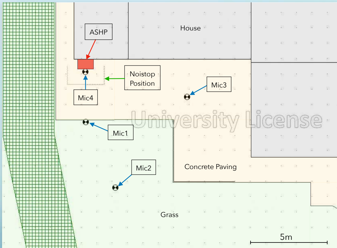
Figure A.1 - Export from CadnaA demonstrating an arial view of the outdoor test location.
