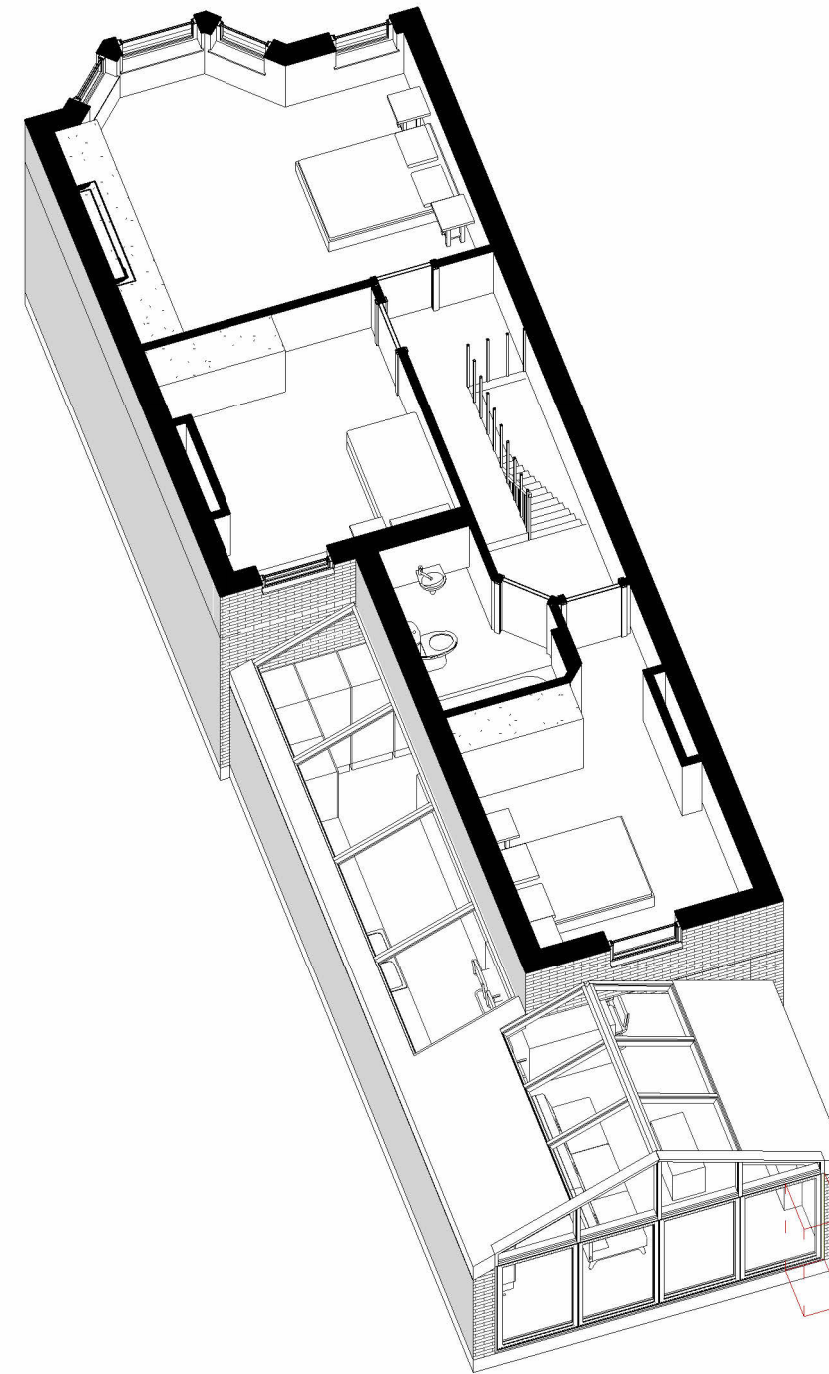
2 Proposed 3D FF
