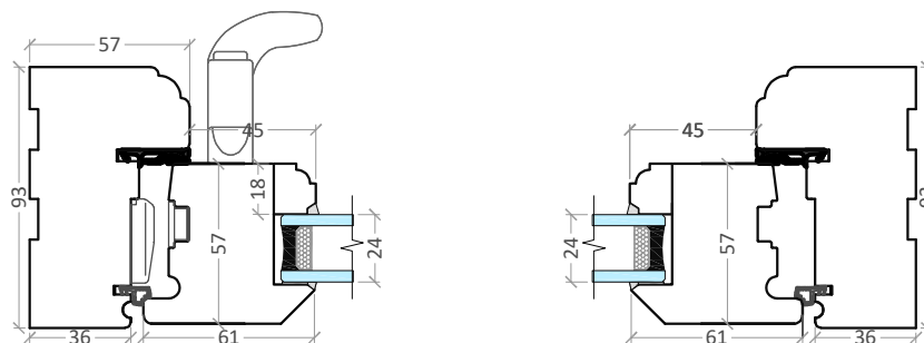
Casement Flush window. 24 DGU. Silicone finish
