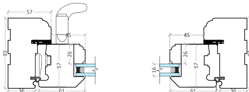
Casement Flush window. 16 DGU. Silicone finish
