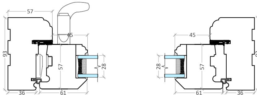
Casement Flush window. 28 DGU. Silicone finish
