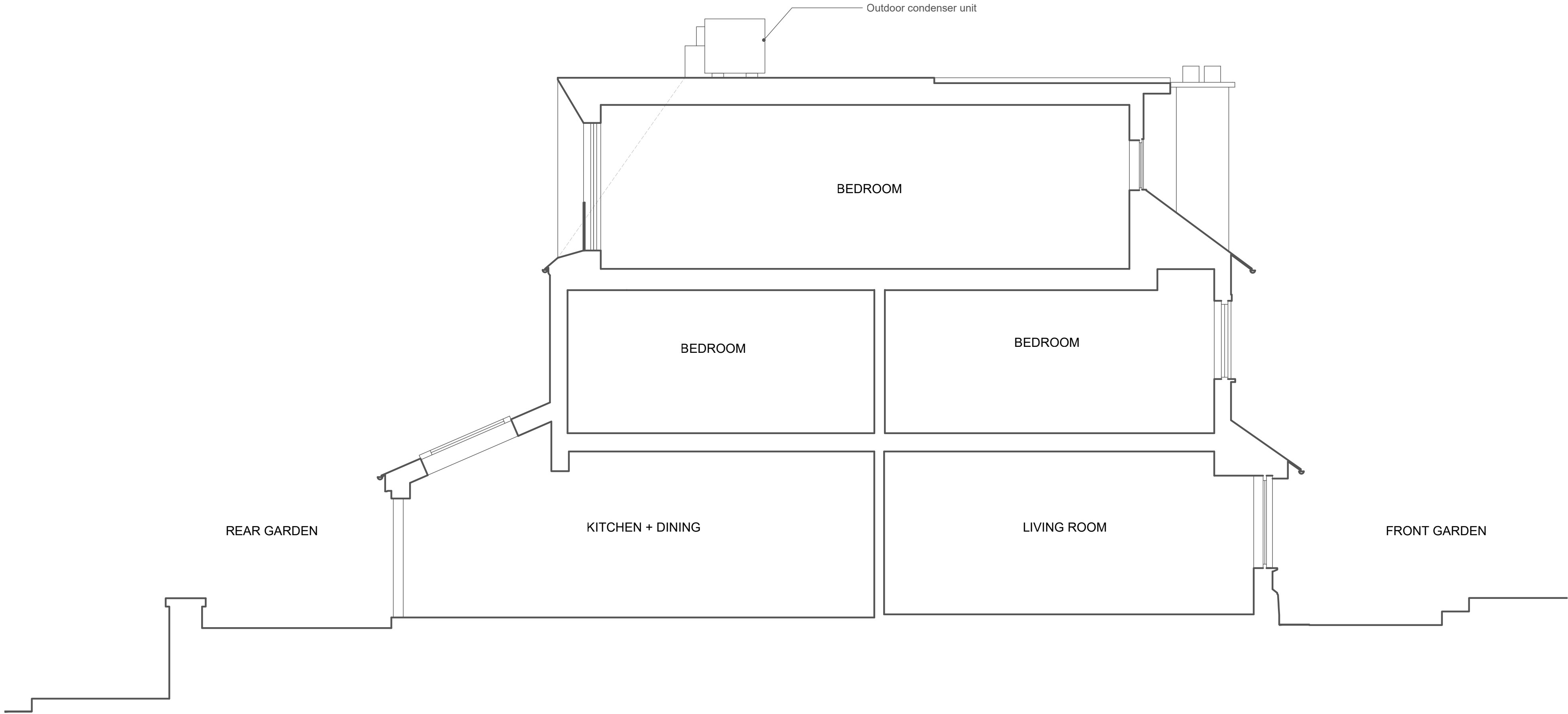
Proposed Section AA 1:50
