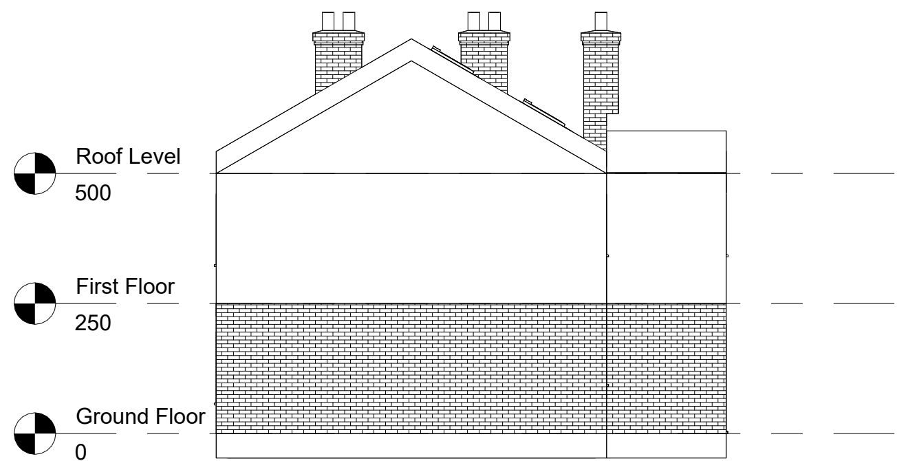
2 West Existing - 1 : 100
