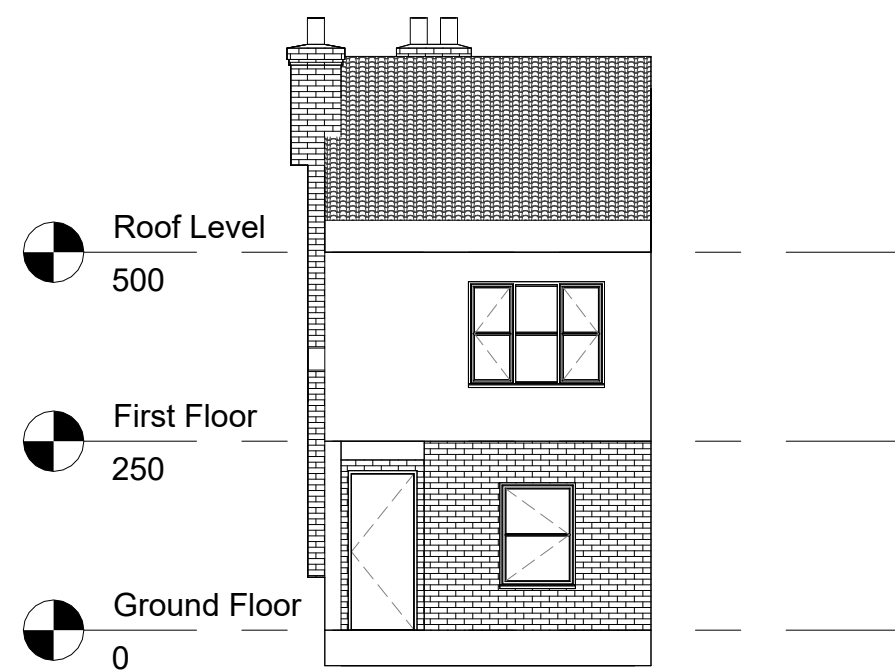
4 North Existing - 1 : 100
