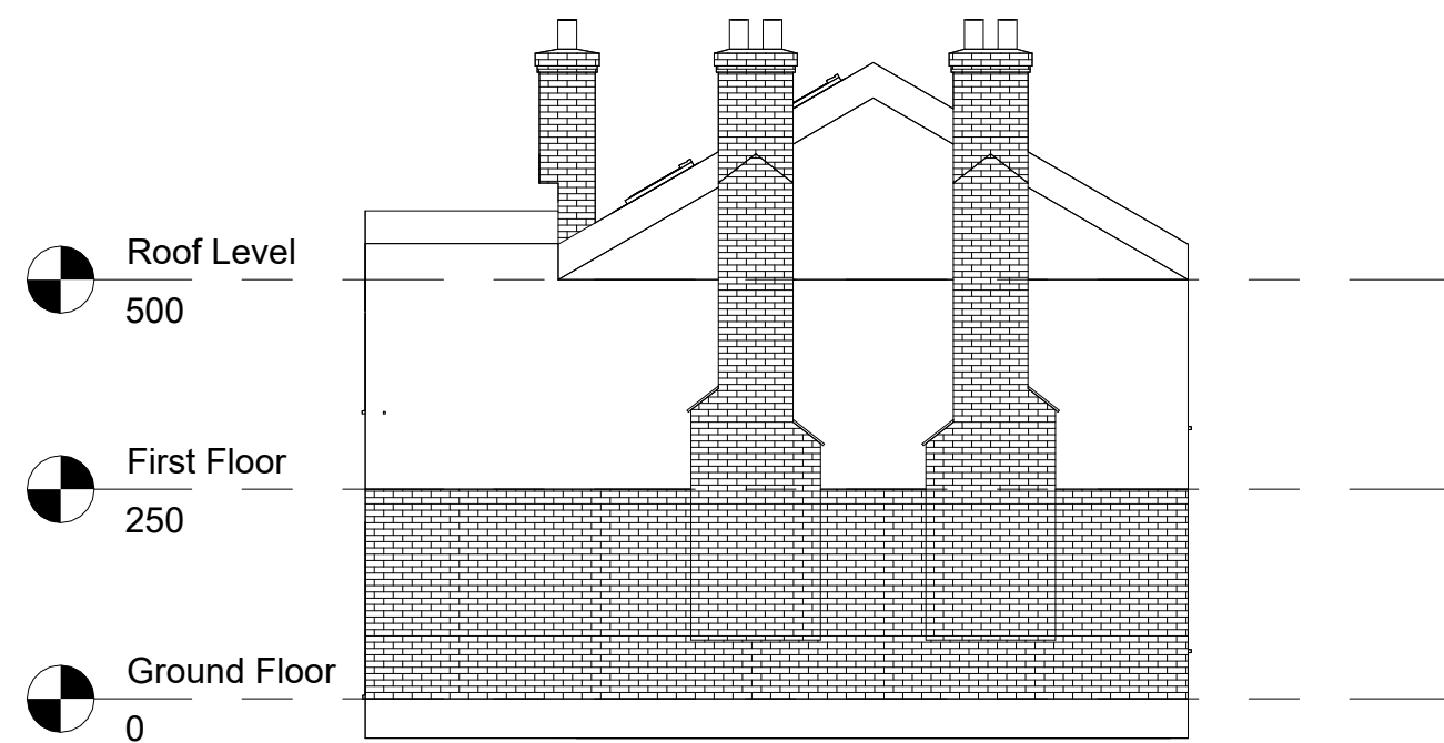
5 East Existing 1 : 100
