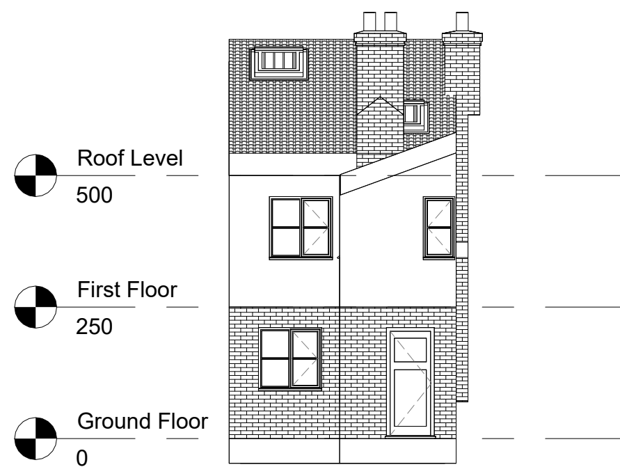
3 South Existing 1 : 100
