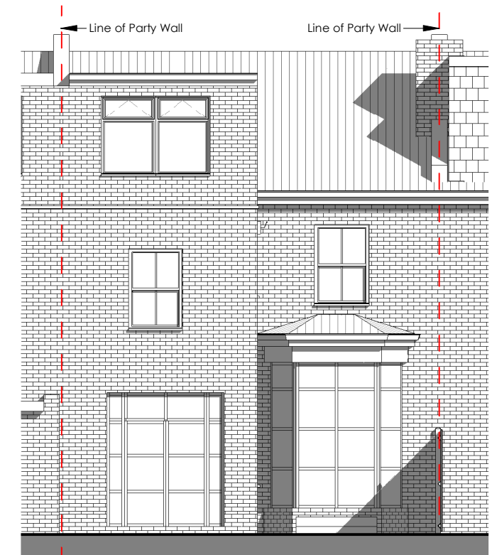
3 Existing Rear Elevation 2620-A-101 1 : 100
