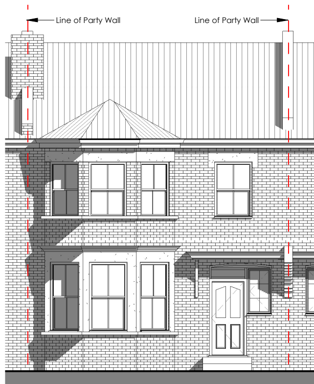
1 Existing Front Elevation 2620-A-101 1 : 100
