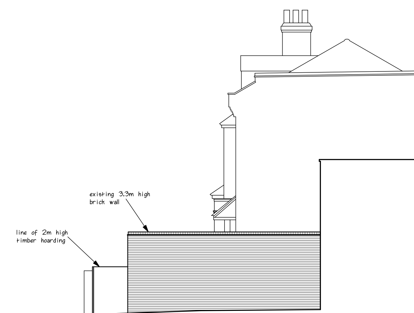
Existing Hoarding Section.
