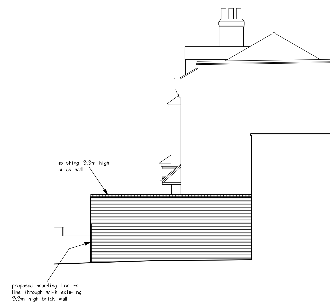
Proposed Hoarding Section.
