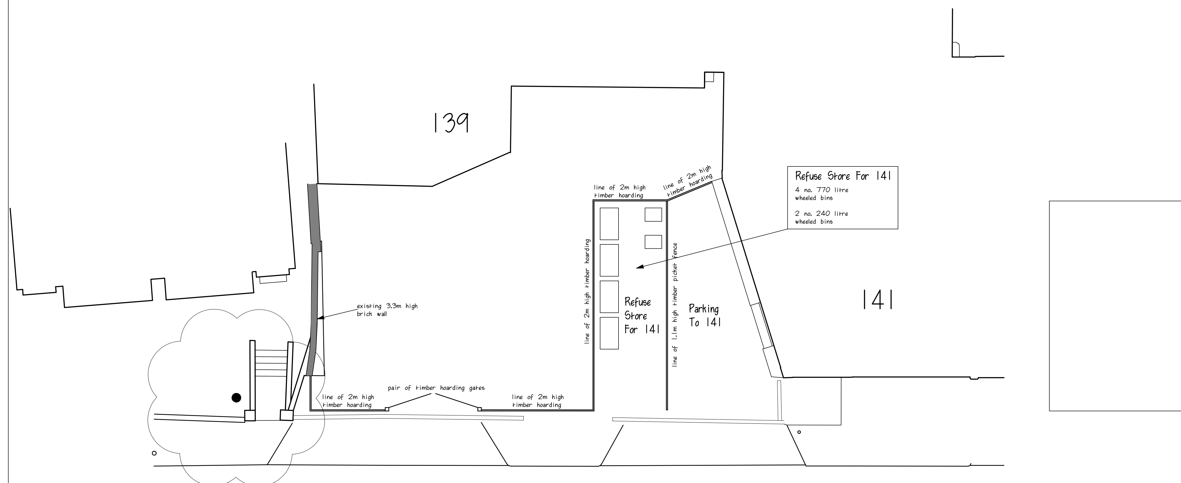
Existing Hoarding Layout.
