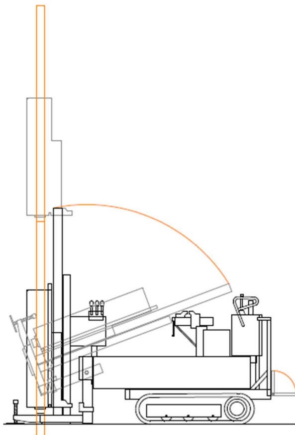
SIDE PROFILE
