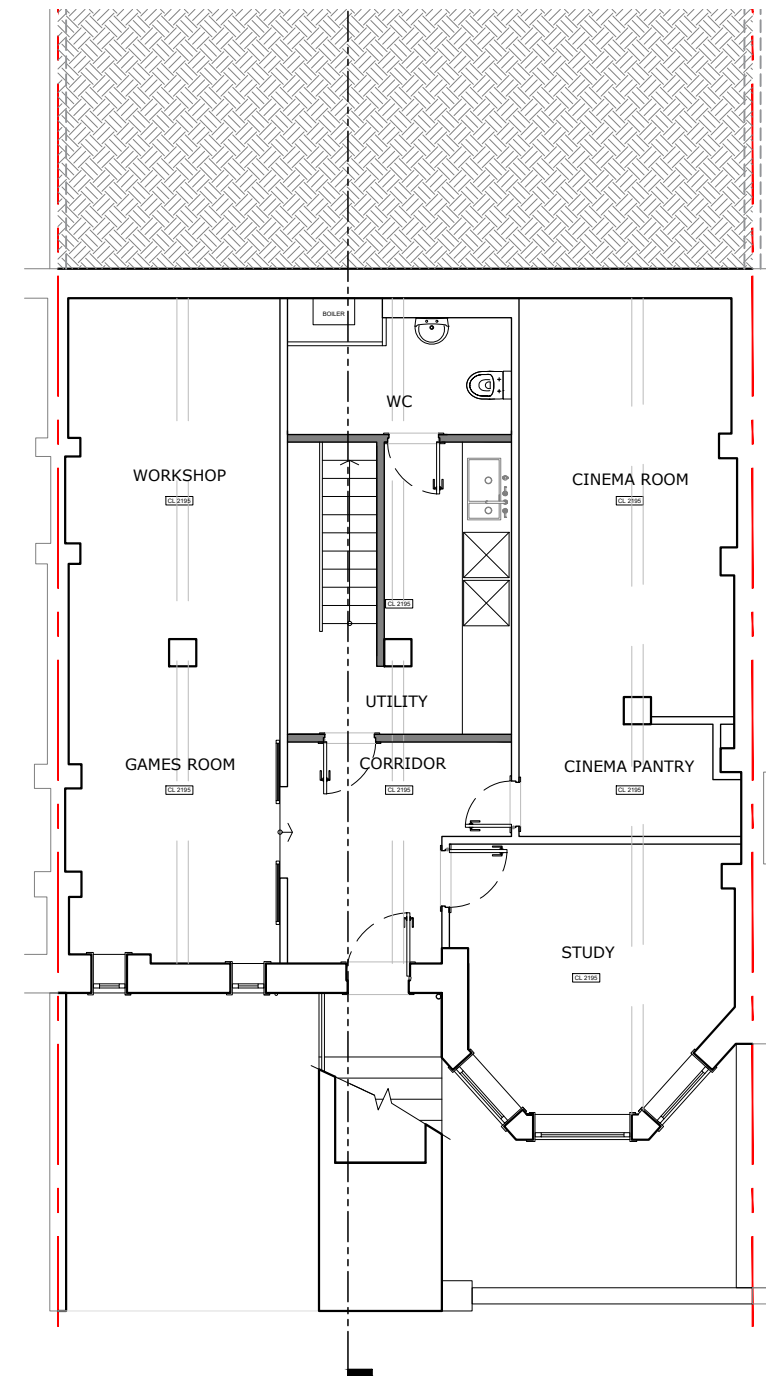
2 Proposed Lower Ground Floor Plan 1 : 100
