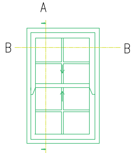
52mm Internal Glazed Slimline Cords & Weights Sliding Casement
