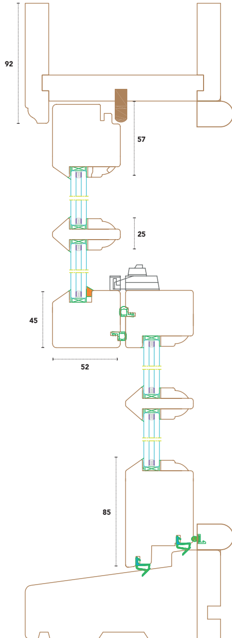
Vertical Section AA
