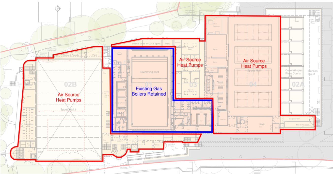
Figure 12 Proposed Heating Systems
