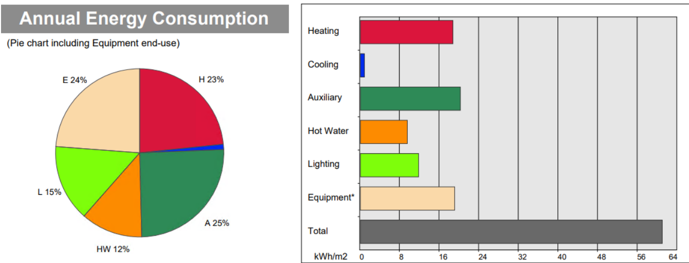
Figure 9 MSC Energy Use (Existing areas)
