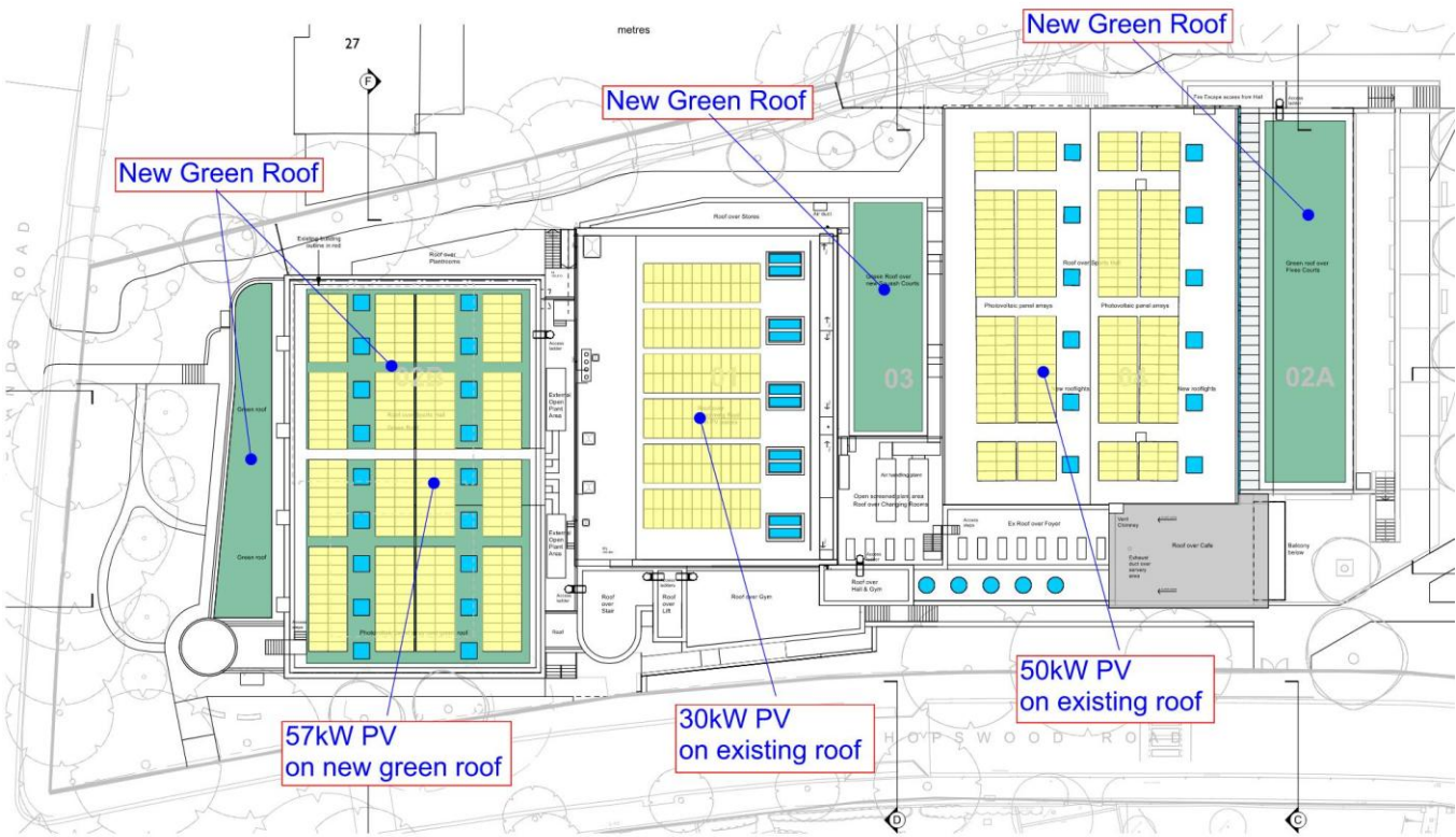
Figure 11 Proposed Location for Renewables
