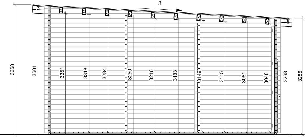
SECTION 1-1
