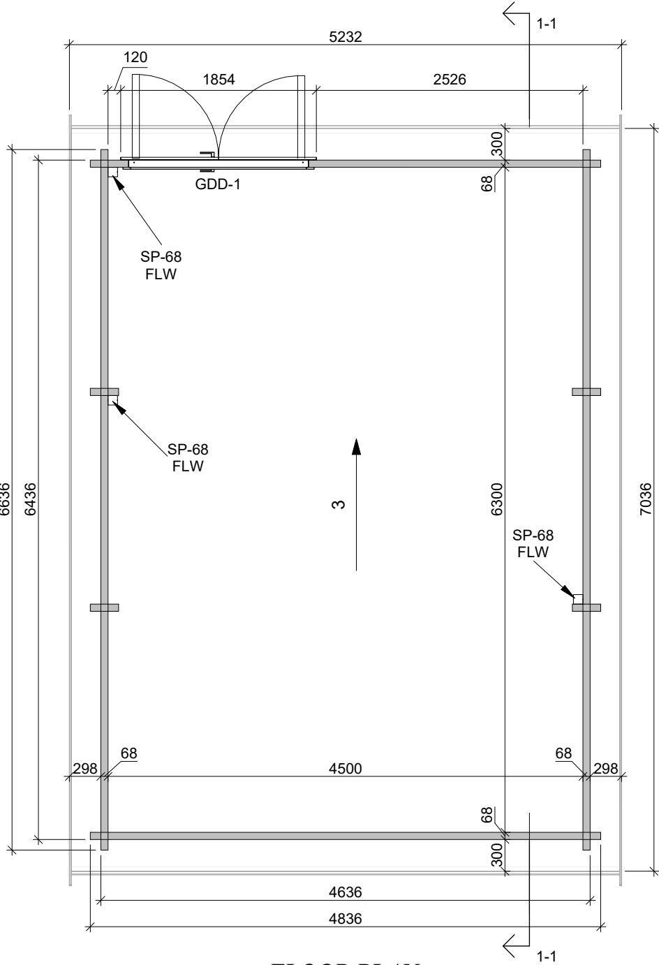
FLOOR PLAN
