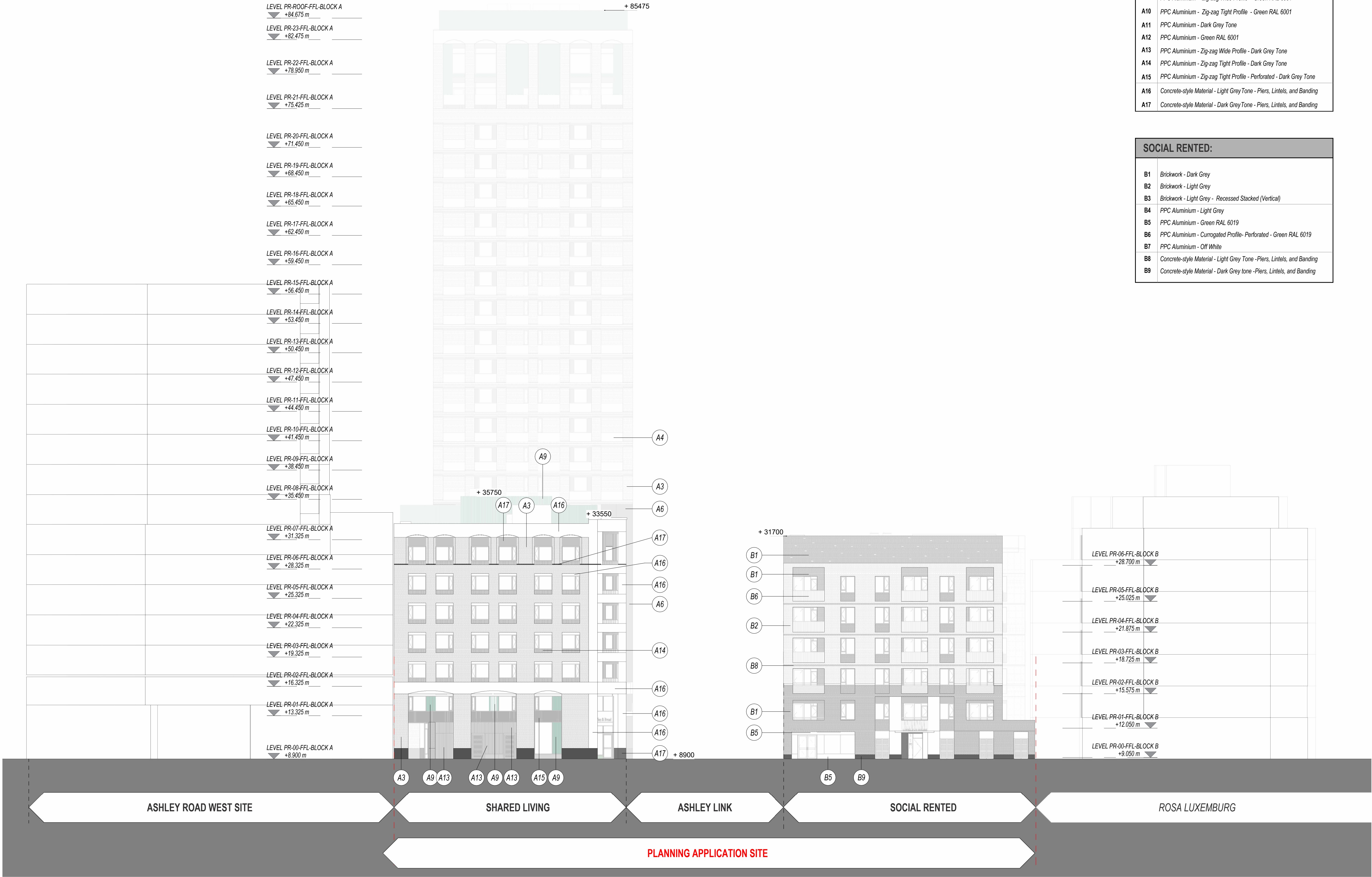
ASHLEY HOUSE SITE - PROPOSED SITE ELEVATION A - ASHLEY ROAD
