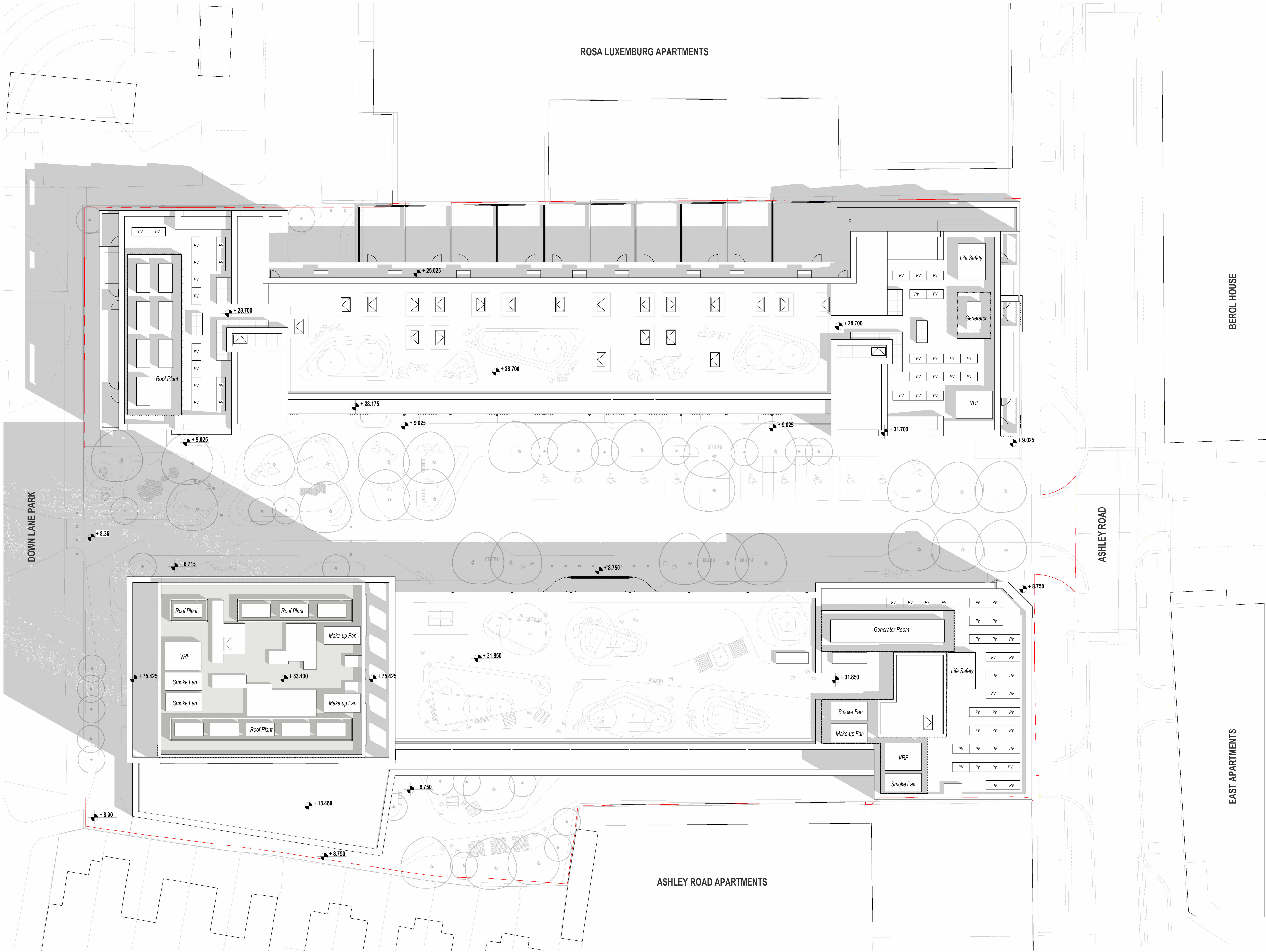
ASHLEY HOUSE SITE - PROPOSED ROOF PLAN 1 : 200
